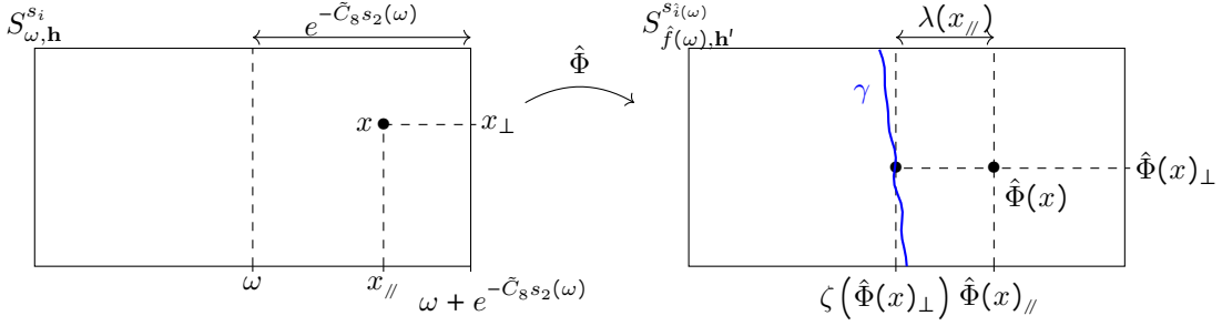
Figure 21: Interpretation of the map \lambda . If x_\parallel = \omega + e^{-\tilde{C}_8 s_2(\omega)} , then \hat{\Phi}(\tilde{x}) is on the right side of \gamma . If x_\parallel = \omega - e^{-\tilde{C}_8 s_2(\omega)} , then \hat{\Phi}(\tilde{x}) is on the left side of \gamma .
