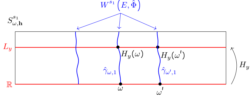
Figure 22: The map H_y .
