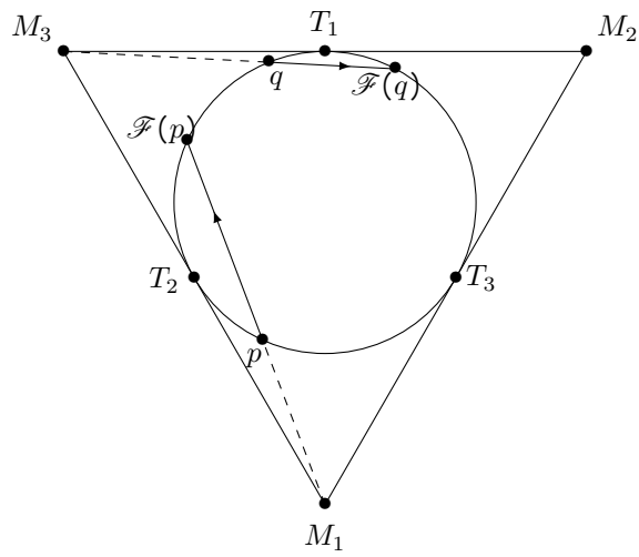
Figure 9: The Kasner map.
