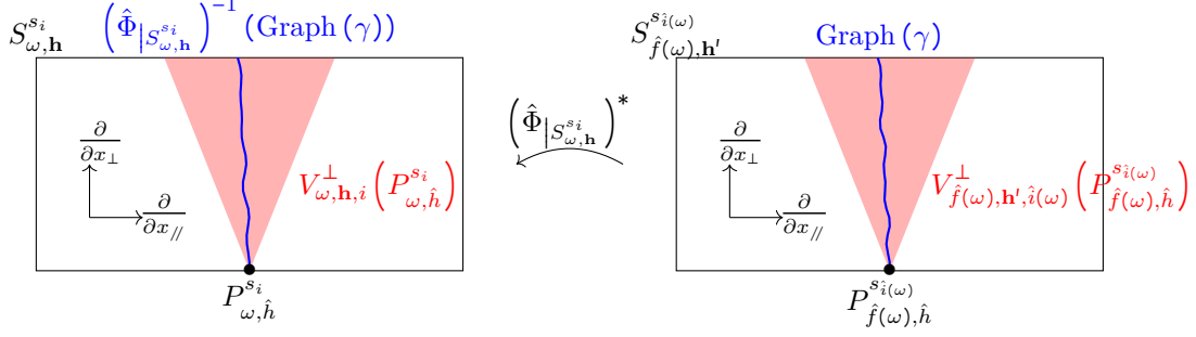
Figure 20: The graph transformation.
