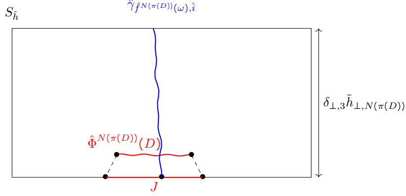
Figure 26: \pi(\hat{\Phi}^{N(\pi(D))}(D)) \subset J with |J| \leq |\hat{\Phi}^{N(\pi(D))}(D)| + \delta_{\perp, 3} \tilde{h}_{\perp, N(\pi(D))} . To avoid clutter, we denote \hat{i} = \hat{i}(\hat{f}^{N(\pi(D))^{-1}}(\omega)) .
