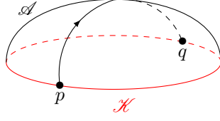
Figure 1: A type II orbit connecting two points of the Kasner circle \mathcal{K} .
