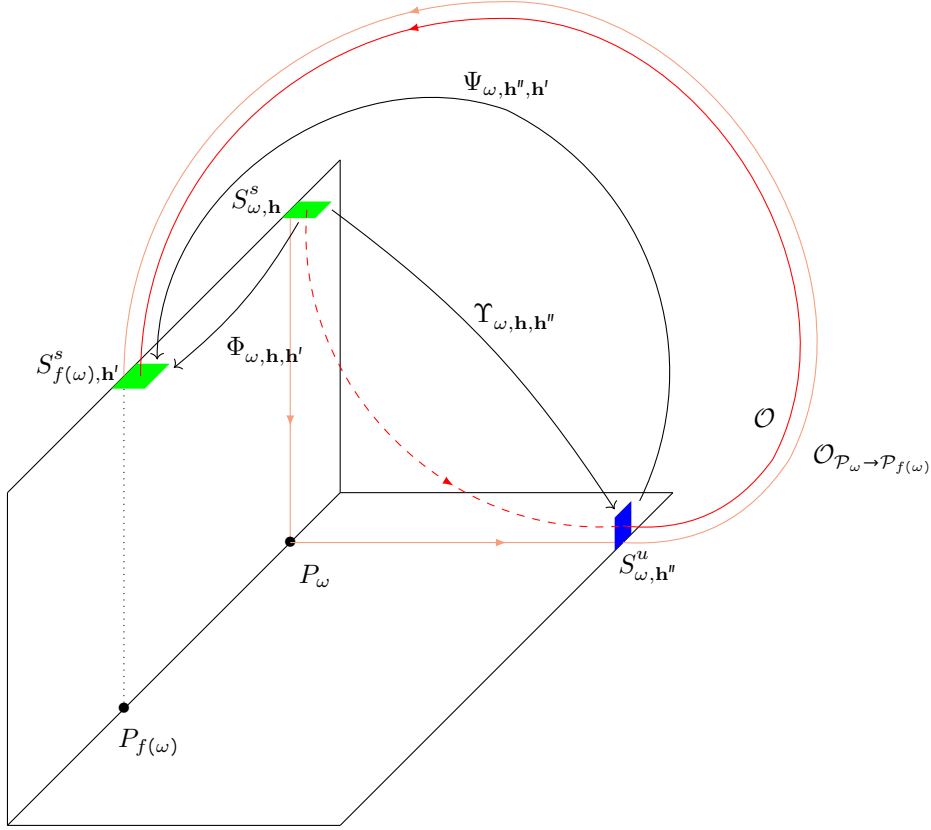
Figure 14: A type IX orbit \mathcal{O} (in red) traveling between the section S_{\omega, \mathbf{h}}^s and the section S_{f(\omega), \mathbf{h}'} . During this travel, the orbit \mathcal{O} stays close to a piece of heteroclinic chain (in melon) passing through the point \mathcal{P}_{\omega} . If the parameters \mathbf{h} , \mathbf{h}' and \mathbf{h}'' are well-chosen (roughly speaking, \mathbf{h}' must be small enough, \mathbf{h}'' much smaller than \mathbf{h}' and \mathbf{h} much smaller than \mathbf{h}' ; explicit bounds will be given in the next sections), the orbit \mathcal{O} will first cross the section S_{\omega, \mathbf{h}''}^u and then cross the section S_{f(\omega), \mathbf{h}'} .
