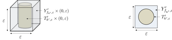
Figure 2: View of the 3D reference cells Y_{k',\epsilon} (left) and the 2D reference cell Y'_{k',\epsilon} (right).
