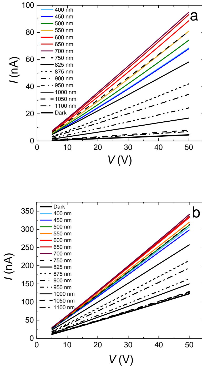
Figure 5. Ohmic parts of V-I characteristics for \text{Ge}_{20}\text{Sb}_{20}\text{S}_{20}\text{Se}_{20}\text{Te}_{20} thin film on \text{Si}/\text{SiO}_2 substrate with interdigitated gold electrodes recorded at 20\text{ }^\circ\text{C} (a) and 75\text{ }^\circ\text{C} (b) under 3.795\text{ mW}/\text{cm}^2 constant power exposure with light of different wavelengths.
