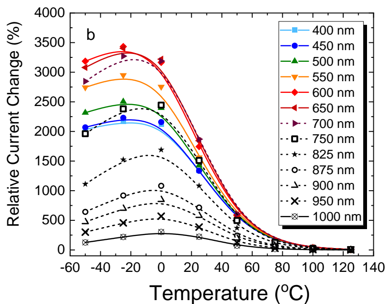
Figure 6. Relative current change as a function of wavelength (a) and temperature (b) measured for \text{Ge}_{20}\text{Sb}_{20}\text{S}_{20}\text{Te}_{20} thin film deposited on \text{Si}/\text{SiO}_2 substrate with interdigitated gold electrodes, using 20 V bias voltage and constant flux ( 1.704 \cdot 10^{16} photons \cdot\text{s}^{-1}\cdot\text{cm}^{-2} ) for the exposure with each wavelength. Curves are drawn as a guide to the eyes.
