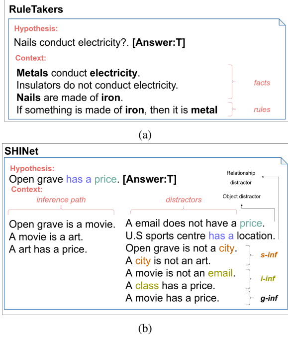
Figure 3: RuleTakers (a) and SHINet 2-hop (b) examples.
