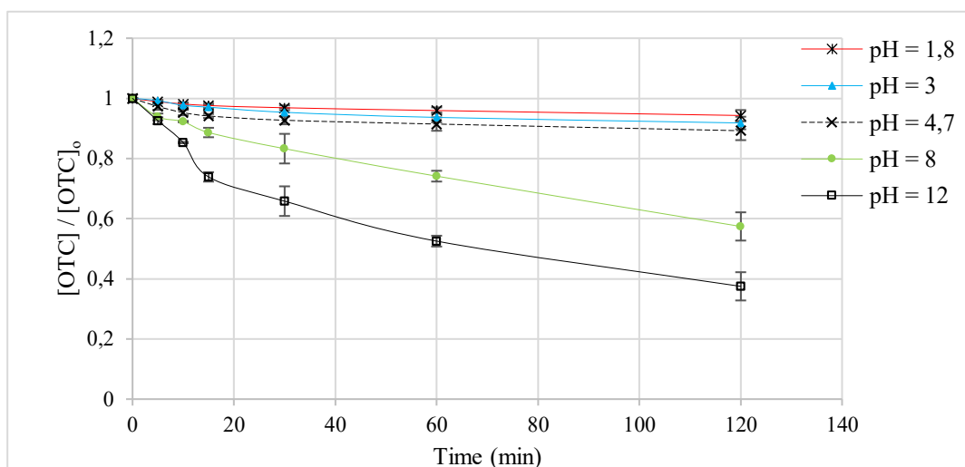
Fig.2 Degradation of OTC at different pH values under UVA light, [OTC] = 10 \text{ mg.L}^{-1}
