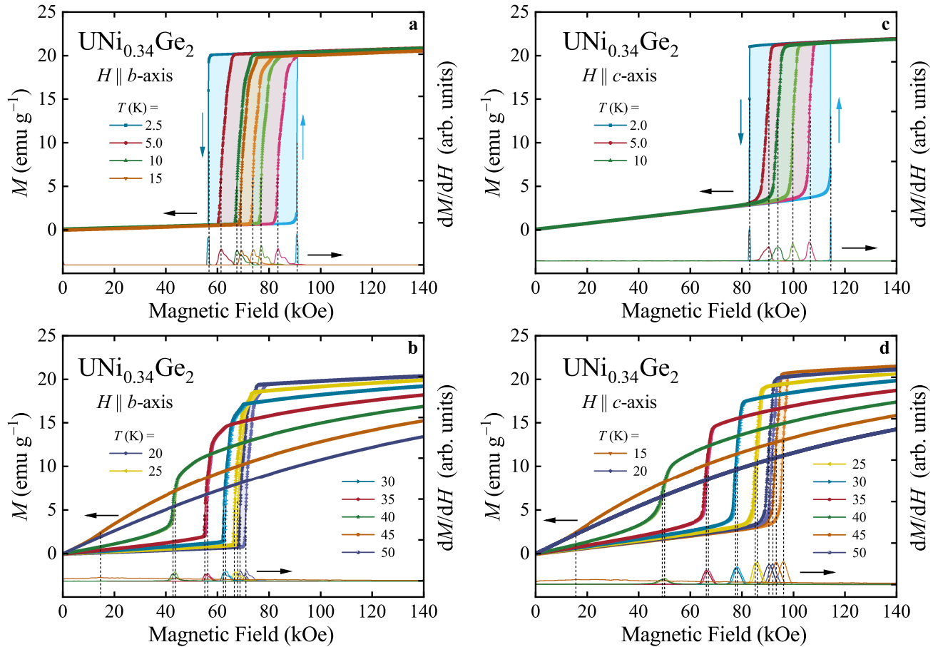
FIG. 6. (Color online) Magnetization of single-crystalline \text{UNi}_{0.34}\text{Ge}_2 measured at various temperatures as a function of (a,b) H \parallel b and (c,d) H \parallel c ; vertical arrows indicate field changes for the largest hysteresis (the arrows for other isotherms are omitted for clarity). Right axes: field derivatives of M(H) ; dashed lines indicate positions of maxima in dM/dH .
