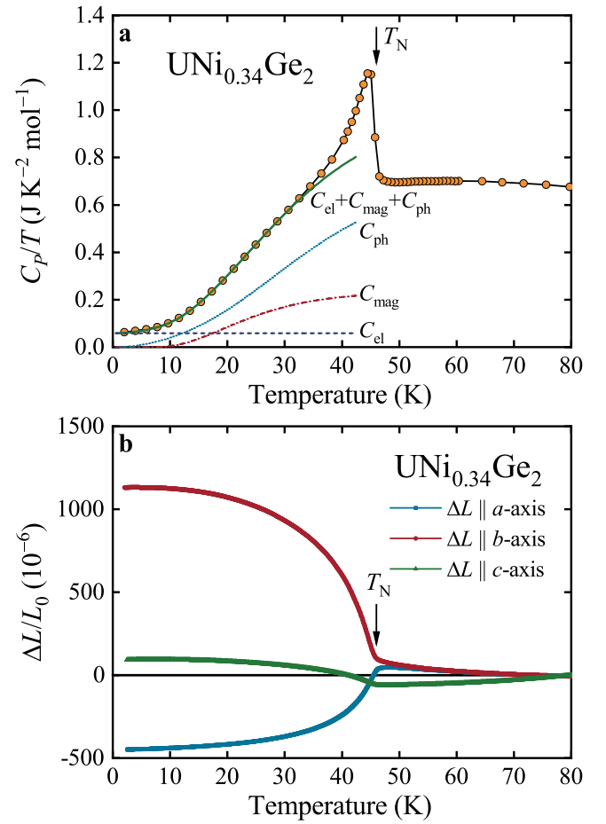
FIG. 4. (Color online) (a) Low-temperature specific heat C_P of single-crystalline UNi 0.34 Ge 2 measured in zero magnetic field and divided by T ; an arrow marks the ordering temperature T_N , and C_{\text{el}} , C_{\text{ph}} and C_{\text{mag}} show – respectively – electron, phonon and magnon contributions to the total C_P/T obtained from least-squares fits (for details see the text). (b) Zero-field and low-temperature linear fractional thermal expansion \Delta L/L_0 of the studied crystal measured along the main crystallographic directions, with L_0 taken at 80 K.
