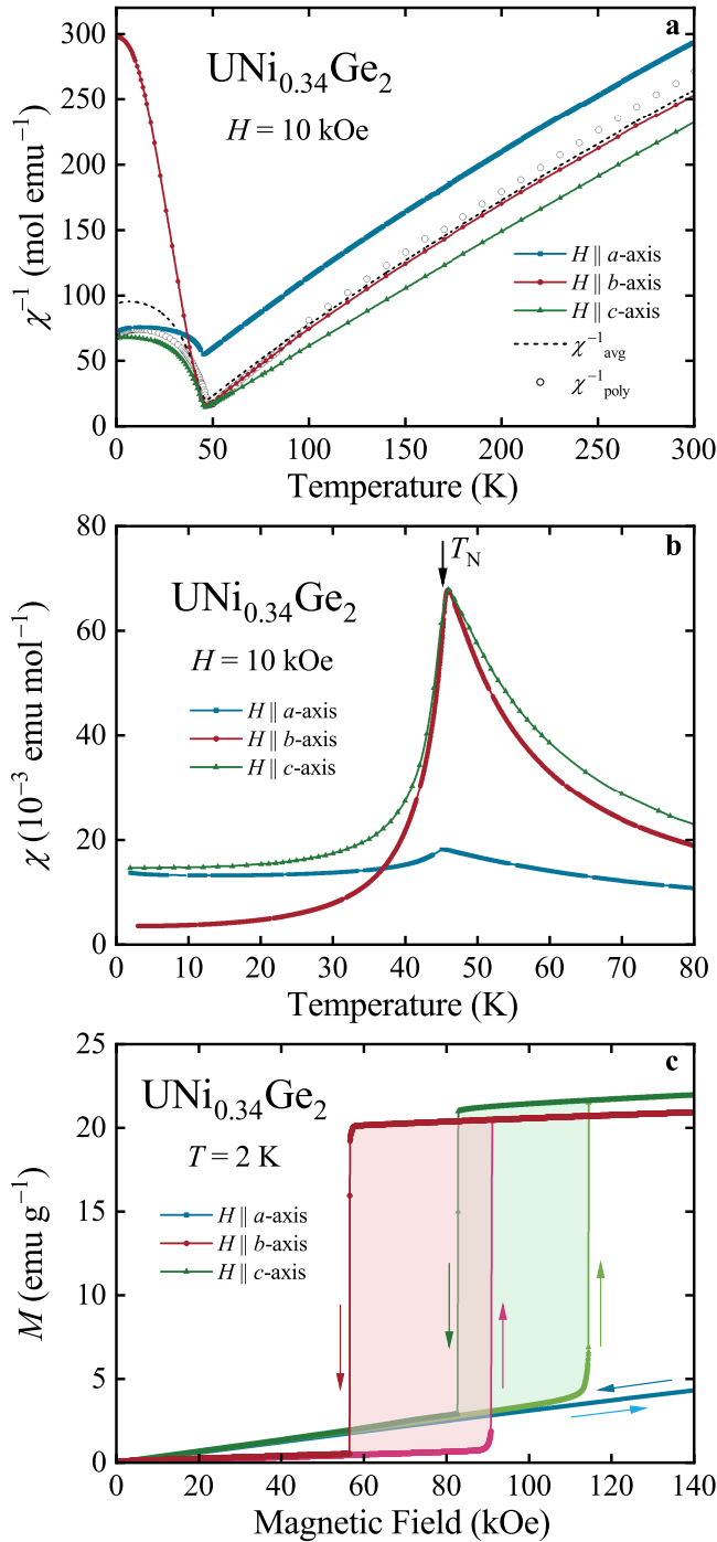
FIG. 3. (Color online) (a) Temperature dependence of inverse magnetic susceptibility \chi^{-1} of single-crystalline UNi 0.34 Ge 2 measured in magnetic field H applied along the main crystallographic axes, together with its averaged values \chi_{\text{avg}} and the data collected earlier for polycrystalline UNi 0.45 Ge 2 [21]. (b) Low-temperature \chi(T) of the crystal studied; an arrow indicates the Néel temperature. (c) Field variation of the magnetization M measured for the main crystallographic axes with increasing and decreasing H , as indicated by arrows.
