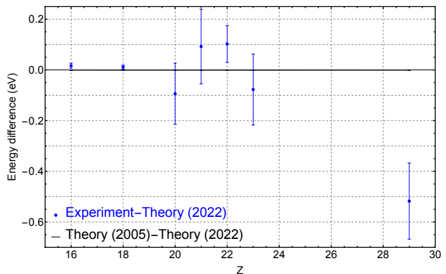
FIG. 7: Comparison between experiment and theory for the 1s2s\ ^3S_1 \rightarrow 1s^2\ ^1S_0 . Z = 16 : this work, Z = 18 [17], Z = 20 : [43], Z = 21 : [44], Z = 22 : [45], Z = 23 : [46], Z = 29 : [20]. Theory (2005): [40], Theory (2022): [41].
