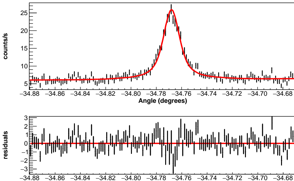
(b) [upper panel] Experimental non-dispersive (parallel) spectrum for the 1s2s\ ^3S_1 \rightarrow 1s^2\ ^1S_0 transition in He-like Sulfur (black points) with 15205 integrated counts, fit with a simulated response function and linear background (red curve) with corresponding reduced- \chi^2 of 1.36. [lower panel] The fit residuals.
