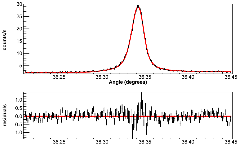
(a) [upper panel] Experimental dispersive spectrum for the 1s2s\ ^3S_1 \rightarrow 1s^2\ ^1S_0 transition in He-like Sulfur (black points) with 68993 integrated counts, fit with a simulated response function and linear background (red curve) with a corresponding reduced- \chi^2 of 1.38. [lower panel] The fit residuals.
