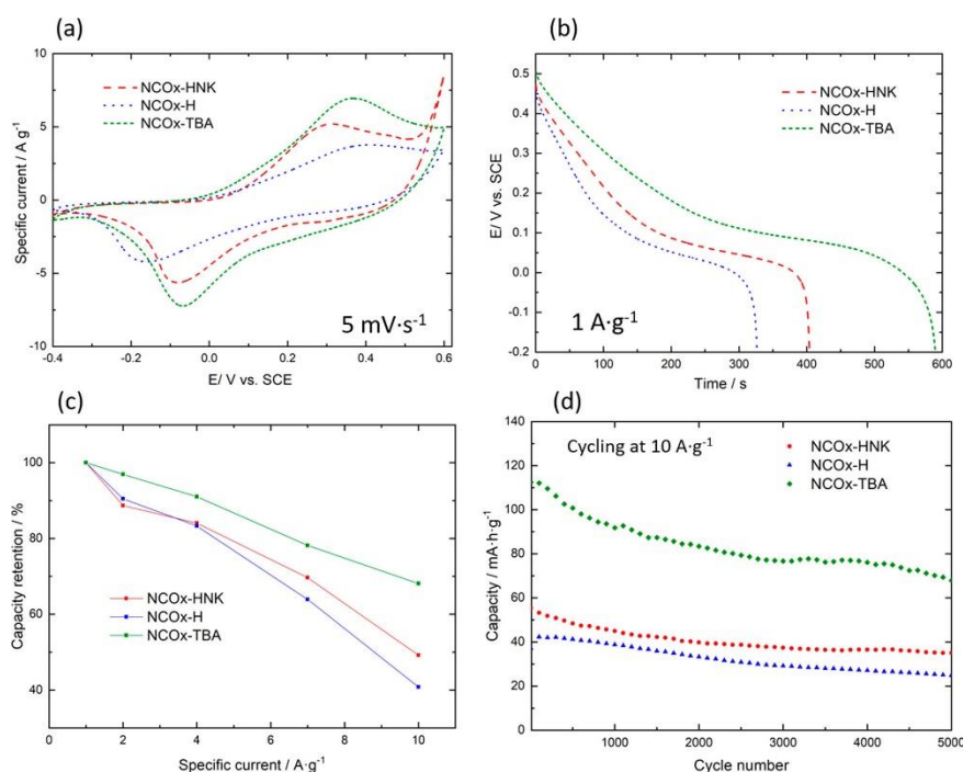
Figure 9. Comparison of the electrochemical response by (a) cyclic voltammetry, (b) galvanostatic discharge, (c) capacity retention at different applied current densities, and (d) capacity retention evaluated by galvanostatic continuous charge–discharge cycling during 5000 cycles at 10 A·g -1 for the different composites obtained during delamination of nickel–cobalt oxyhydroxide by TBA + intercalation in 1M LiOH.
