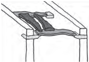
35. The three structural levels of the stone roof in the fort: corbels (light grey) support lintels (mid-grey), supporting in turn another level of lintels (dark grey) (Q. Devers, 2012).
