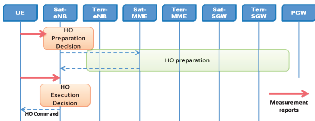
Figure 4. Optimized handover algorithms
