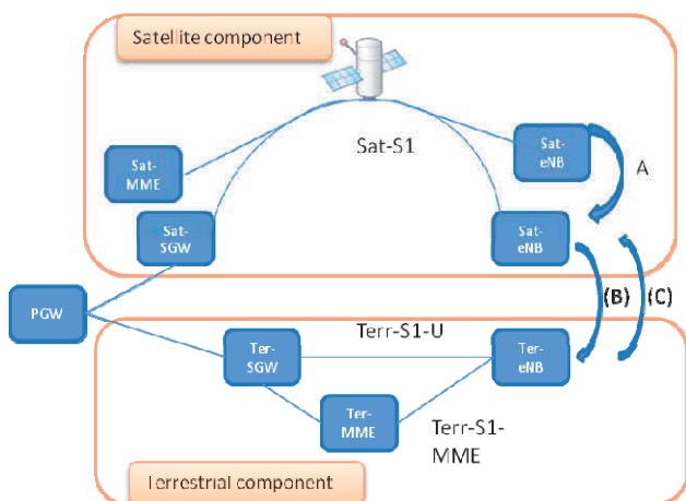
Figure 1. Architecture.
