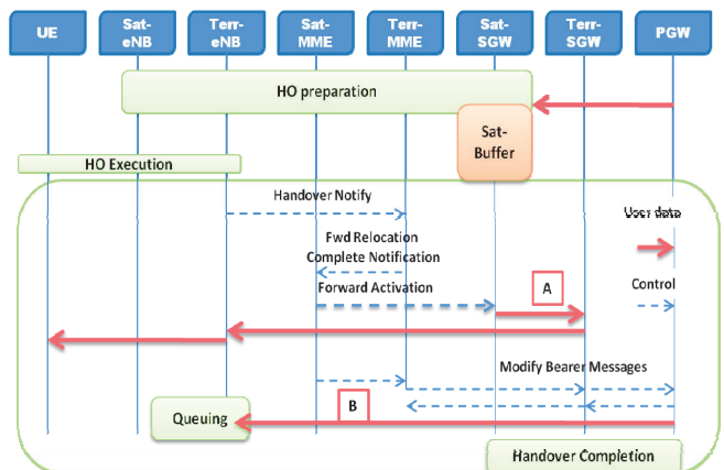
Figure 5. Tunnel forwarding optimization
