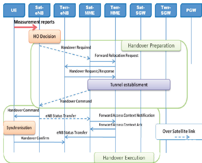
Figure 2. HO preparation and execution
