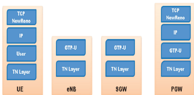
Figure 6. User plane for NS3 simulation
