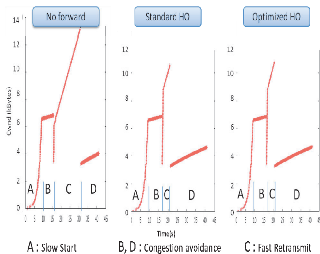
Figure 7. TCP congestion windows evolution
