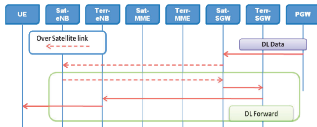
Figure 3. Standard tunnel forwarding
