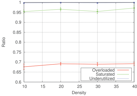
Fig. 2. Packet Delivery Ratio (PDR) vs Car Density
