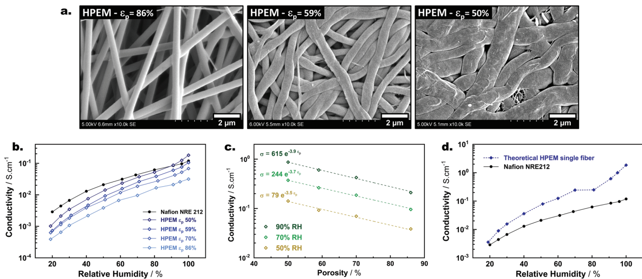
Figure 2. Properties of pressed HPEM according to their porosity \epsilon_p : a) SEM images; b) evolution of proton conductivity with relative humidity at 80 °C; c) evolution of proton conductivity with \epsilon_p at 80 °C; d) extrapolated conductivities for a perfectly dense HPEM versus relative humidity at 80 °C.
