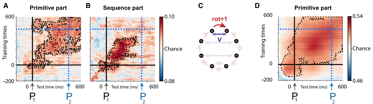
Figure 5. Decoding primitives
