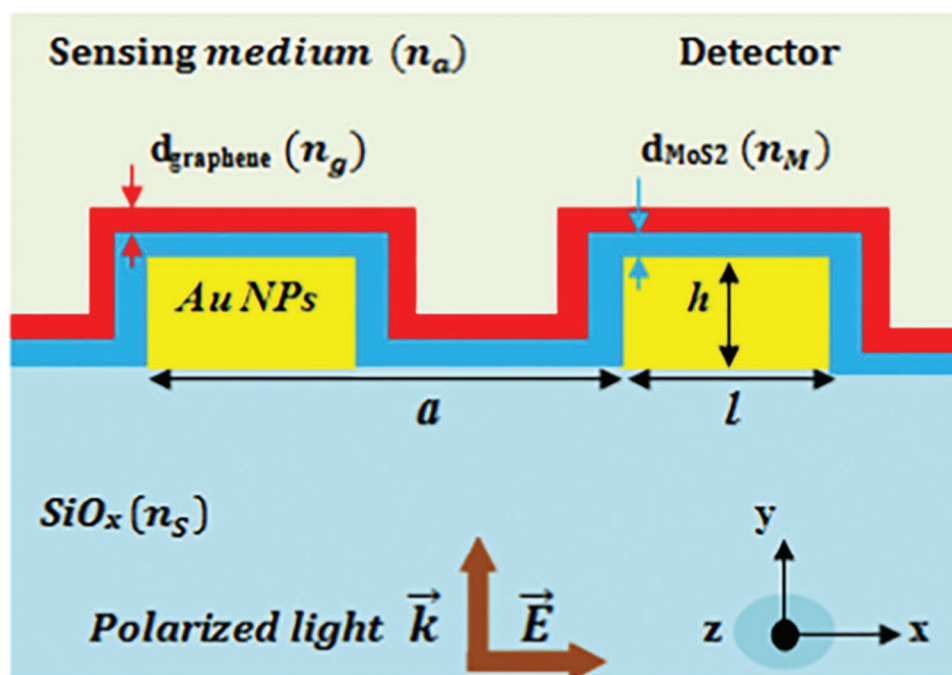
Figure 16. Schematic representation of AuNPs when covered with few layers of MoS 2 /graphene and another dielectric lying on top (detection medium of refraction index n_a ) and deposited on a SiO x substrate (SiO x /AuNPs/MoS 2 /graphene/dielectric). The particles form a 1D grating along x -axis. The AuNPs grating is characterized by parameter h referring to the particle's height, l is their length, and a is the lattice parameter. The input wave source (monochromatic plane wave) is also shown. Reproduced with permission. [172] Copyright 2020, Elsevier Ltd. Besides the theoretical study of sensing DNA hybridization, an experimental work on a D-shaped fiber SPR sensor based on a CVD MoS 2 /CVD graphene was developed for the detection of glucose. Reproduced with permission. [175] Copyrights 2020, Elsevier B. V. They functionalized graphene with pyrene-1-boronic acid (PBA) via \pi - \pi stacking interactions to realize the selectivity and utilized gold film to excite the SPR effect. In addition, the sensitivity of the sensors is dependent on the number of MoS 2 layers. In this work, the as-obtained biosensor with three-layer MoS 2 and monolayer graphene demonstrated the highest sensitivity of 6708.87 nm RIU -1 , as well as good selectivity of glucose against UA, AA, and DA with a concentration of 0.1 mM.
