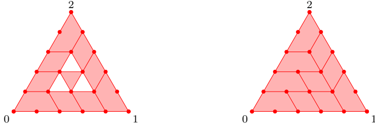
Fig. 8: Not minimal (left) and minimal (right) degrees of freedom for \mathcal{P}_{5-k}\Lambda^k(T) , where T is a 2-simplex.
