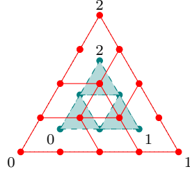
Fig. 6: Internal small edges chosen using the map \gamma .
