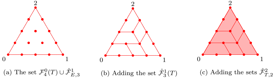
Fig. 9: Minimal degrees of freedom for \mathcal{P}_{4-k}\Lambda^k(T) , where T is a 2-simplex.
