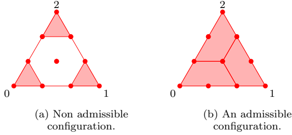
Fig. 4: Two cellular complexes
