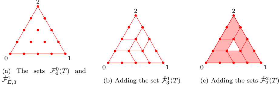
Fig. 7: Construction of not minimal degrees of freedom for \mathcal{P}_{4-k}A^k(T) , where T is a 2-simplex.
