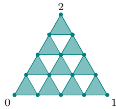
Fig. 2: Overdetermining degrees of freedom for \mathcal{P}_4^- \Lambda^k(T) , where T is a 2-simplex.
