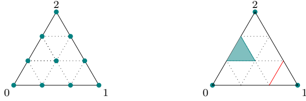
Fig. 1: Example of small k -simplices, k = 0 (left) and k = 1, 2 (right), for r = 3 . The nodes of the principal lattice of degree r in T coincide with the small nodes. In blue the small triangle s^{(1,0,1)} , in red the small edge s^{(0,2,0)} .
