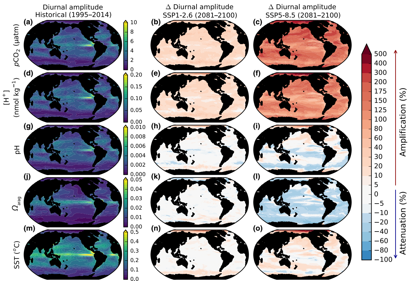
FIGURE 4 The simulated mean diurnal amplitudes of pCO_2 , [H^+] , pH, \Omega_{arag} , and SST and their changes under SSP1-2.6 and SSP5-8.5. The simulated mean modern (1995–2014) diurnal amplitudes of pCO_2 , [H^+] , pH, \Omega_{arag} , and SST and their change in 2081–2100 under SSP1-2.6 and SSP5-8.5 relative to the historical period.
