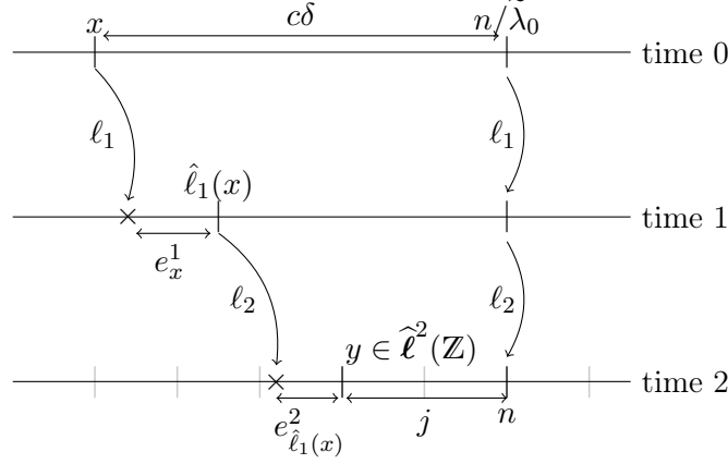
FIGURE 2. Computation of the cumulated difference c\delta in the case k = 2 . The point y is the biggest point of \ell^2(\mathbb{Z}) smaller than n .
