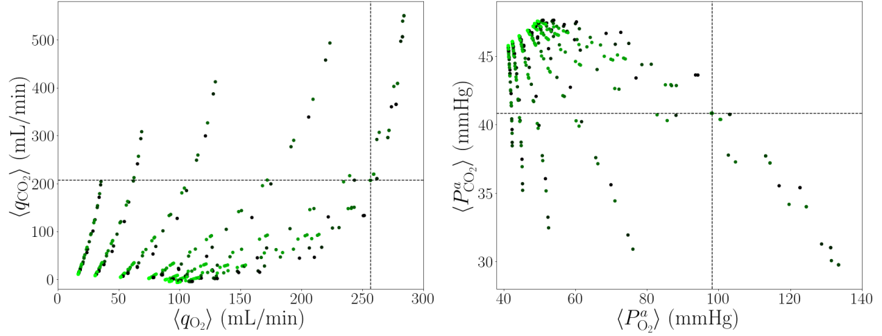
FIGURE 14. Plots with averaged (a) fluxes of \text{O}_2 and \text{CO}_2 , (b) arterial partial pressures of \text{O}_2 and \text{CO}_2 , with green-scaled values of E .
