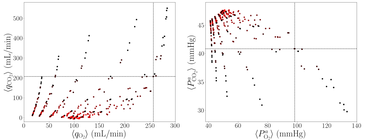
FIGURE 15. Plots with averaged (a) fluxes of \text{O}_2 and \text{CO}_2 , (b) arterial partial pressures of \text{O}_2 and \text{CO}_2 , with red-scaled values of R .
