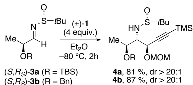
Scheme 2. Reactions with imines ( S,R S )- 3a,b
