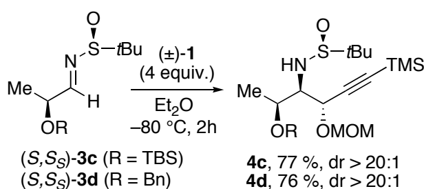
Scheme 3. Reactions with imines ( S,S_S )- 3c, d
