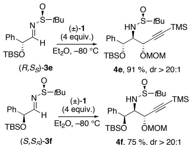
Scheme 4. Reaction with imines ( R,S_S )- 3e and ( S,S_S )- 3f
