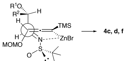
TS2 (anti-Felkin) : R 1 = TBS, Bn; R 2 = Me, Ph
