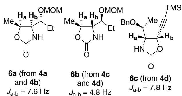
Figure 2. Oxazolidinones 6a-c for stereochemical correlations.
