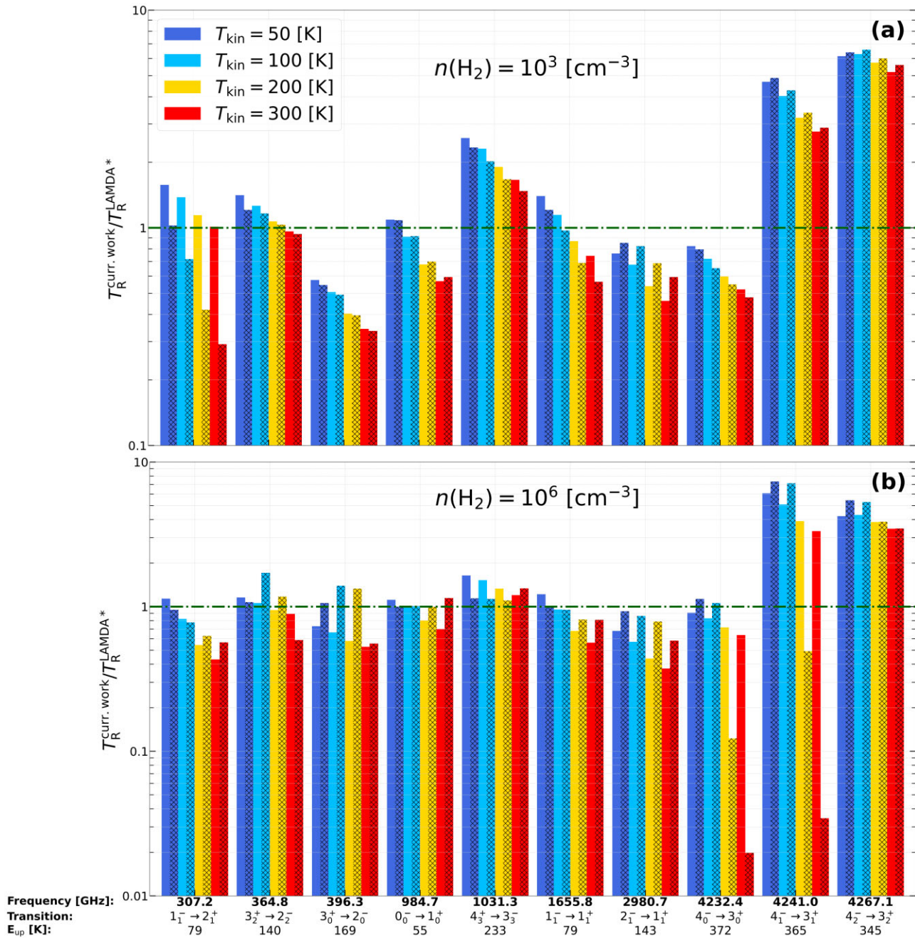
Figure 1. [Correction to fig. 6 originally published by Demes et al. (2022)] The relative ratio of radiation temperatures at 50, 100, 200, and 300 K kinetic temperatures for the majority of the observed radiative \text{H}_3\text{O}^+ transitions calculated for diffuse [panel (a), n(\text{H}_2) = 10^3 \text{ cm}^{-3} ] and dense [panel (b), n(\text{H}_2) = 10^6 \text{ cm}^{-3} ] molecular cloud conditions. The T_R^{\text{curr.work}} data is computed from our new set of rate coefficients, while the T_R^{\text{LAMDA}^*} set is calculated based on the corresponding collisional data from the LAMDA data base. The colour bars correspond for radiative transfer calculations in the optically thin environments ( N = 10^{13} \text{ cm}^{-3} ), while the hatch-filled bars show the same quantities, but for optically thick regions ( N = 10^{16} \text{ cm}^{-3} ).
