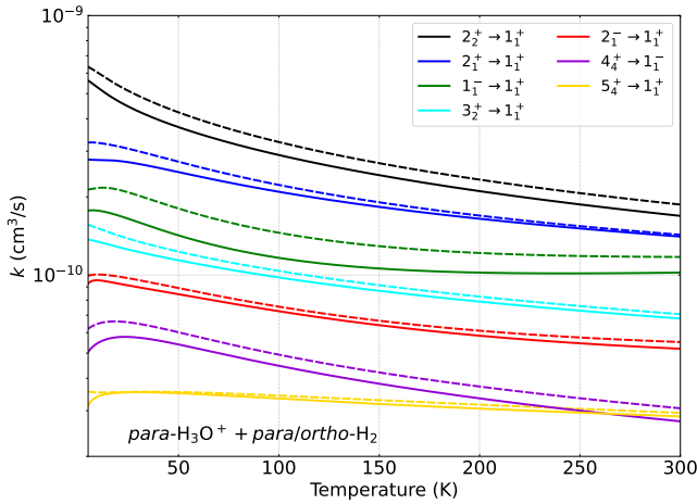
Figure 4. Kinetic temperature dependence of the rate coefficients for the same rotational transitions as shown in Fig. 2 for p\text{-H}_3\text{O}^+ collision with p\text{-H}_2 (solid lines) and o\text{-H}_2 (dashed lines) projectiles.
