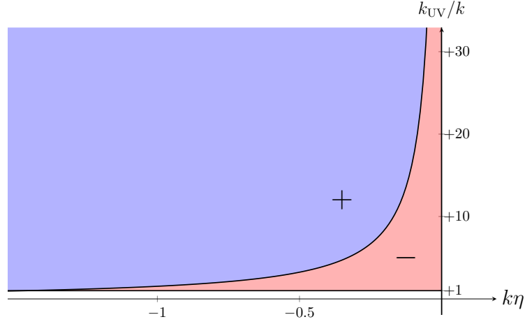
Figure 3. A plot of the sign of \text{Re } \mathfrak{Q}_{\mathbf{k}} as a function of k\eta and \kappa = k_{\text{UV}}/k (for the case k\eta_{\text{in}} \rightarrow -\infty ), with blue representing positive and red being negative. The boundary between the two signs follows roughly the curve k_{\text{UV}}\eta \simeq \sqrt{3} .
