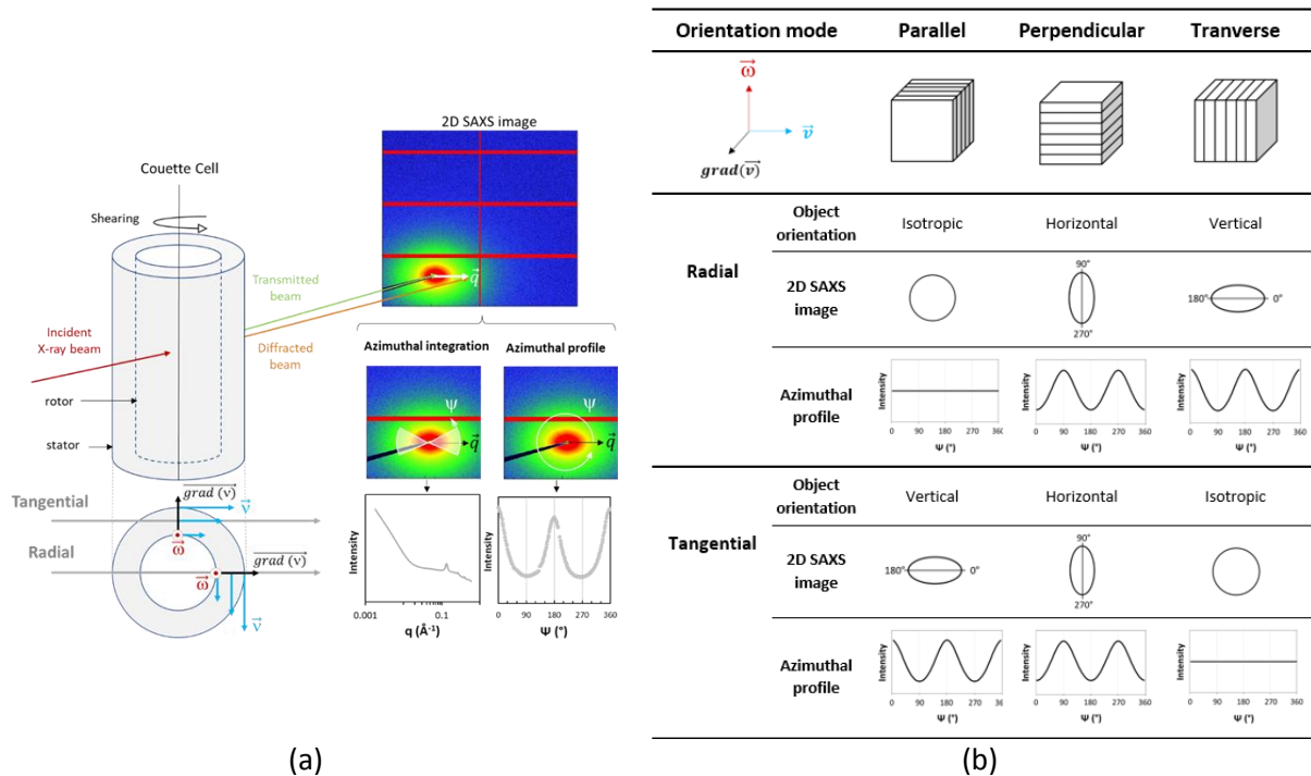
Figure 3 : (a) Rheo-SAXS measurement principle and schematic representation of 2D SAXS image treatment (b) Schematic representation of the 2D SAXS image in radial and tangential configuration corresponding to the three possible orientations of the lamellar domains
