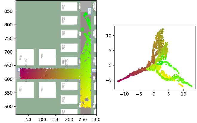
Fig. 6. Spatial distribution of the UEs in the test set ( left ) and their corresponding learned chart obtained on the fly ( right ). Color is added to distinguish local neighborhoods.
