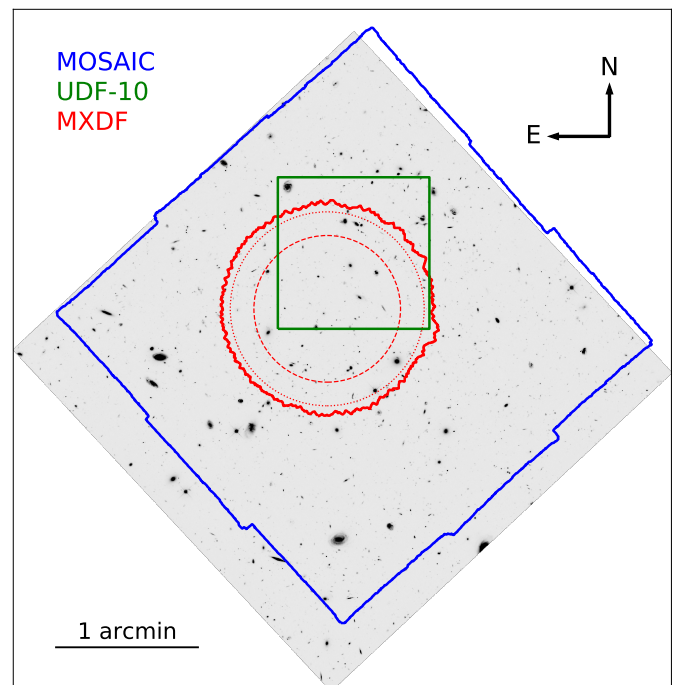
Fig. 2. Location of the three deep fields used in this paper: MXDF (141-h depth), MOSAIC (10-h depth), and UDF-10 (31-h depth) overlaid on the HST F775W UDF image. The dotted and dashed red circles show the MXDF 10- and 100-h exposure time isocontours, respectively.
