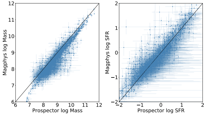
Fig. 34. Comparison of the Prospector and Magphys stellar mass and SFR results for the SED fits of all MUSE galaxies identified in the R15 catalog.
