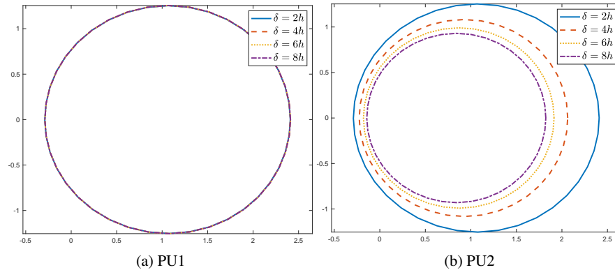
Fig. 2: Numerical range of the preconditioned operator ( \mathbf{a} = [-x, -y]^T ).
