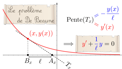
Figure 2: Animation of De Beaune’s problem (find a curve such that the distance between the vertical projection of any of its points to the intersection of its tangent with the x -axis is constant). In the video, the point (x, y(x)) is moving, and the text and relevant lines (some not shown here) appear step by step.
