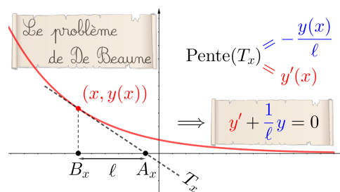
Figure 2: Animation of De Beaune’s problem (find a curve such that the distance between the vertical projection of any of its points to the intersection of its tangent with the x -axis is constant). In the video, the point (x, y(x)) is moving, and the text and relevant lines (some not shown here) appear step by step.
