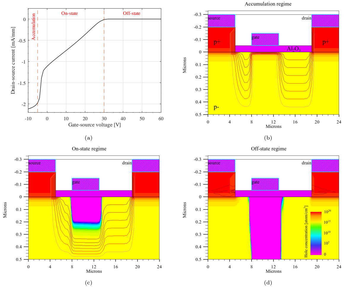
Figure 3: (a) Drain current vs. Gate voltage at T = 450 K. Hole concentration and current flowlines in (b) the accumulation mode at V_{gs} = -10 V, (c) in the on-state mode at V_{gs} = 10 V and (d) in the off-state mode at V_{gs} = 40 V.
