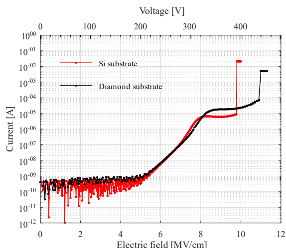
Figure 10: Current versus electric field characteristics for 50 \times 50 \mu\text{m}^2 MIM capacitor on diamond and silicon substrates.
