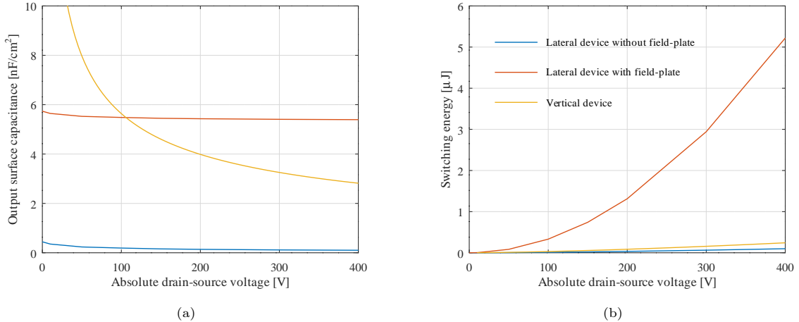
Figure 8: (a) Output surface capacitance and (b) the corresponding switching energy according to the drain-source voltage for various device architectures : one vertical architecture and two lateral devices with and without the presence of a field-plate.
