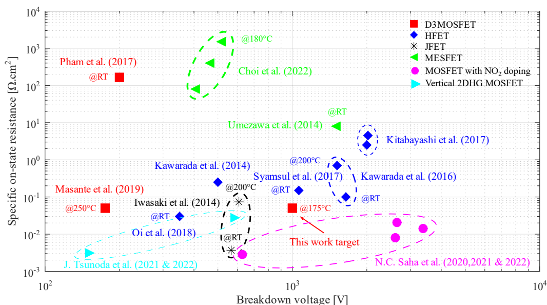
Figure 1: Specific on-state resistance vs. breakdown voltage performances of power diamond FETs reported in the literature. Experimental points are taken from [5, 6, 7, 8, 9, 10, 11, 12, 16, 17, 18, 19, 20, 21]
