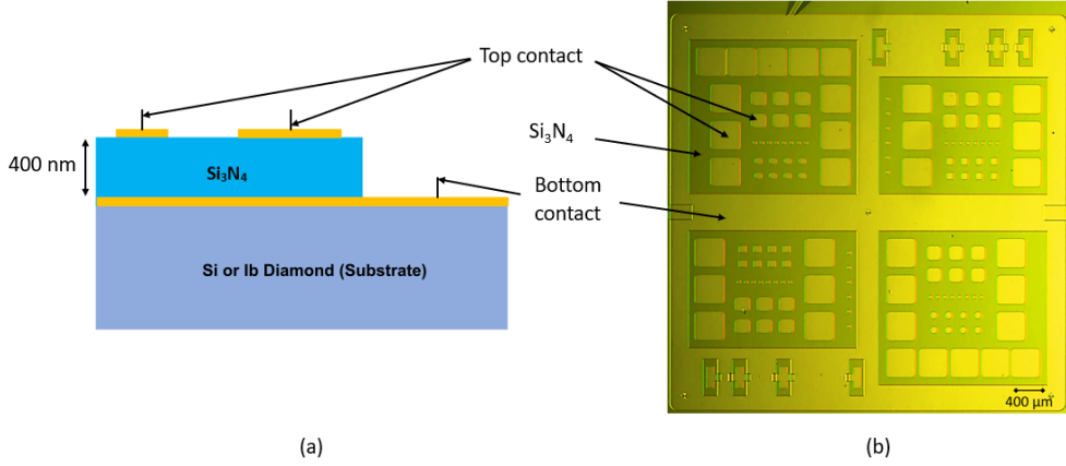
Figure 9: Design of MIM capacitors : (a) Schematic cross-section of MIM capacitors, (b) MIM capacitor device optical micro-graph.
