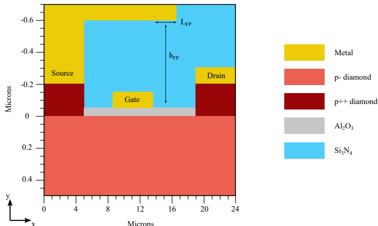
Figure 5: Schematic of a source-field-plate D3MOSFET with a passivation layer made of \text{Si}_3\text{N}_4 .
