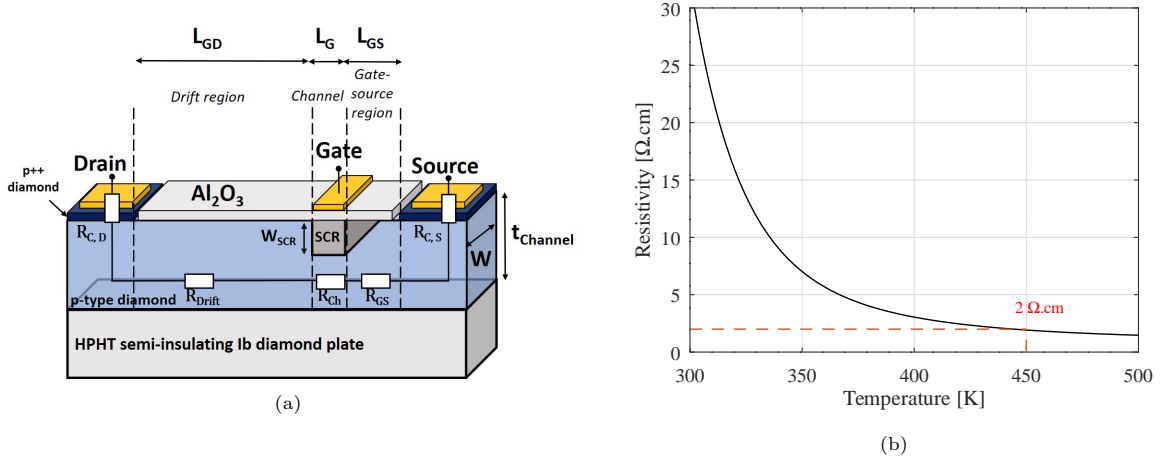
Figure 2: (a) Schematic cross-section of a deep-depletion diamond MOSFET (D3MOSFET) and (b) Resistivity according to the temperature for a D3MOSFET with a boron-doped channel at N_a = 8 \cdot 10^{16} \text{ atom}\cdot\text{cm}^{-3} and a compensation level in donor atoms of N_d/N_a = 4 \% .
