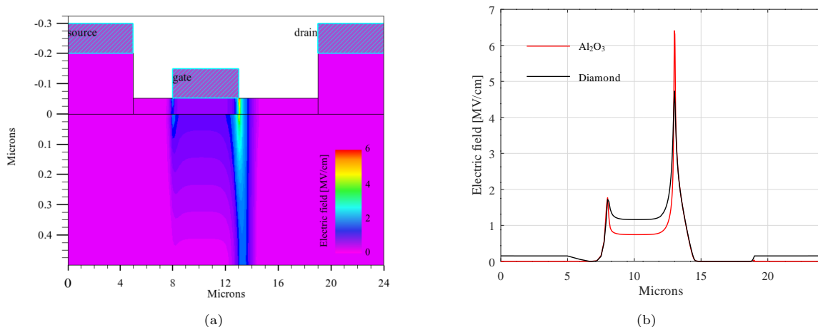
Figure 4: (a) Finite element simulation of the electric field distribution in the off-state with a drain bias of -200 V and a gate bias of 40 V. (b) The lateral electric field profiles on the oxide surface (red) and the top surface of the diamond (black) are extracted from the simulation.
