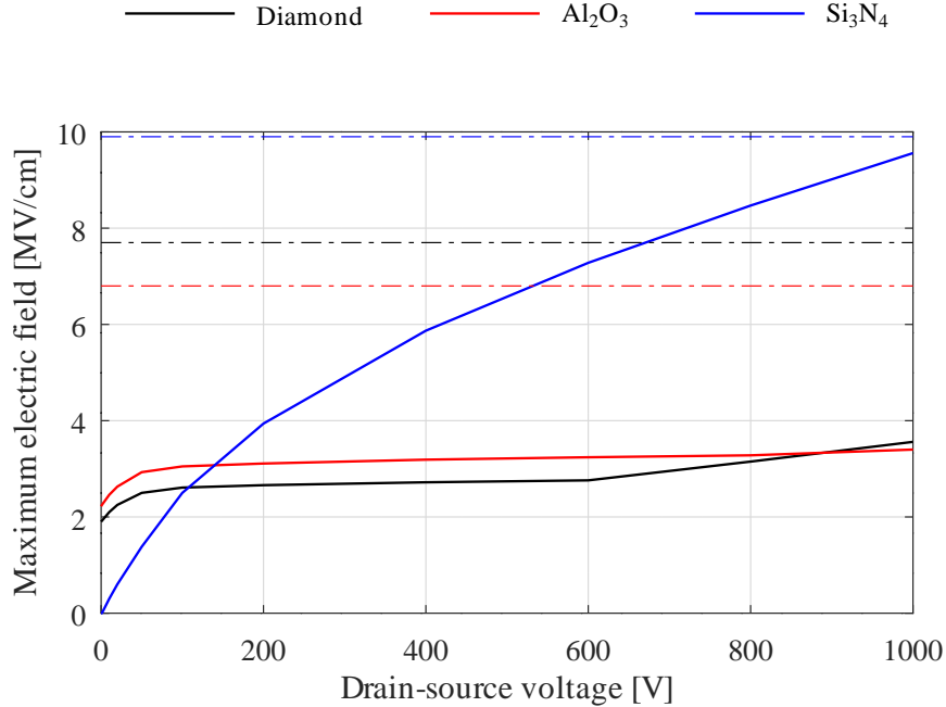
Figure 7: Maximum electric field evolution along the V_{ds} within the diamond (black curve), the gate-oxide (red curve) and the passivation layer (blue curve) for a source-field-plate. Is also displayed in dashed lines, the theoretical critical electric field of each material.
