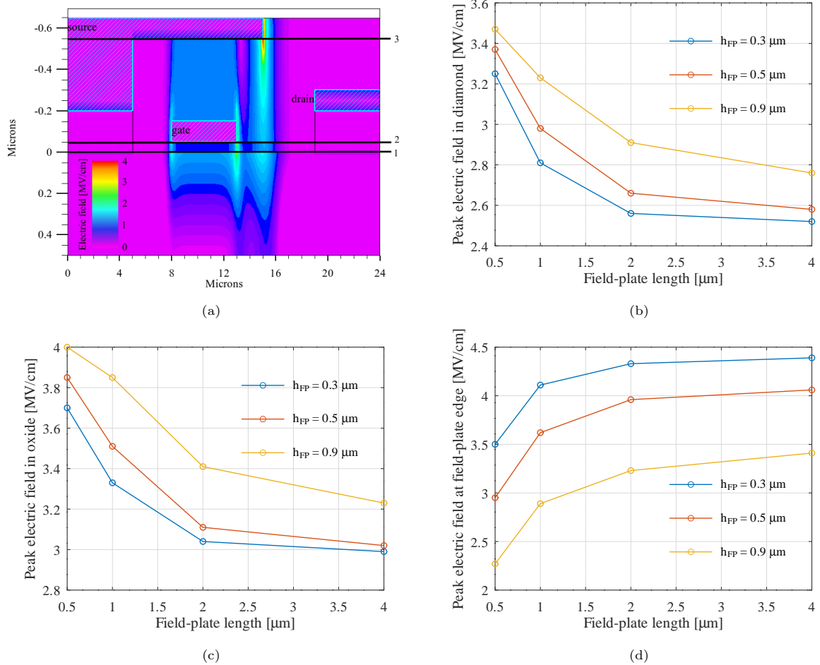
Figure 6: (a) Finite element simulation of the electric field distribution in the off-state with a drain bias of -200 V and a gate bias of 40 V with highlighted lateral cutlines. Electric field evolution according to the drain extension of the field-plate for different field-plate heights in (b) the diamond cutline, (c) the gate-oxide cutline and (d) the field-plate edge cutline.
