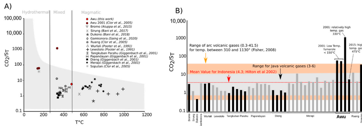
Figure 7. (A) Variation of the CO_2/S_T ratios as a function of temperature for the Indonesian volcanoes. The diagram discriminates the magmatic gas signature (Merapi, Bromo, Dukono, Sirung, Wurliali, and Lewotolo) from the hydrothermal (low-temperature fumarole at Awu and Sopotan) and mixed gases composition (Papandayan, Dieng, Tangkuban Parahu, Ruang, and the high-temperature gas from Awu). (B) The CO_2/S_T ratios highlight the strong CO_2 signature of Awu above the means value of Indonesian volcanoes and above the arc volcanic gases. Awu CO_2 signature is also higher than the Java arc, considered as the CO_2 -enriched arc [4,55].
