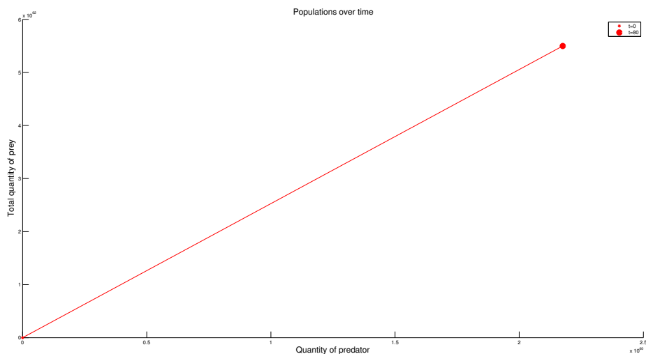
Figure 4: Unbounded solution
