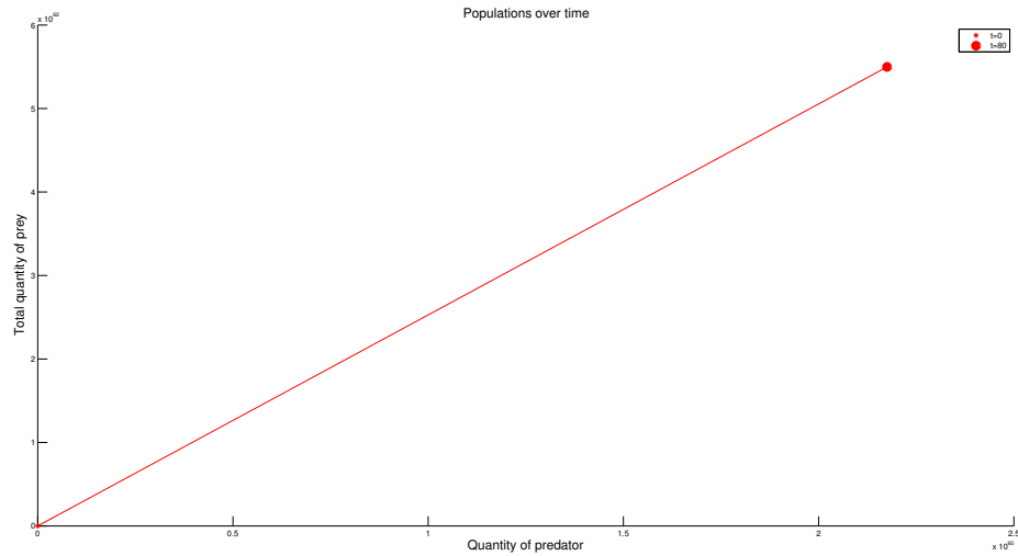
Figure 4: Unbounded solution
