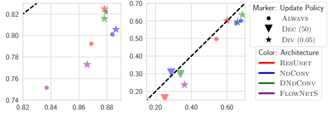
Figure 5: MOTION-F1 on recent (x) and older data (y) on stream A (left) and B (right). DIV policy (with l = 0.05 ) yields improvements in most of the cases. Some low-performance configurations are out of the scope of the plot.
