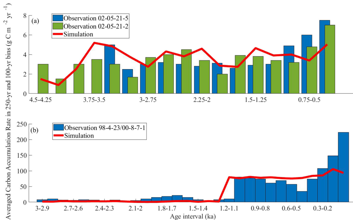
Figure 7. Simulated and observed carbon accumulation rates from 4.5 ka to 2014 CE (0 ka) in 250-year bins in subtropical region for (a) sawgrass and from 3 ka to 2014 CE (0 ka) in 100-year bins for (b) sawgrass and tree island. The transition from sawgrass to tree island was assumed according to the observation (Jones et al., 2014).
