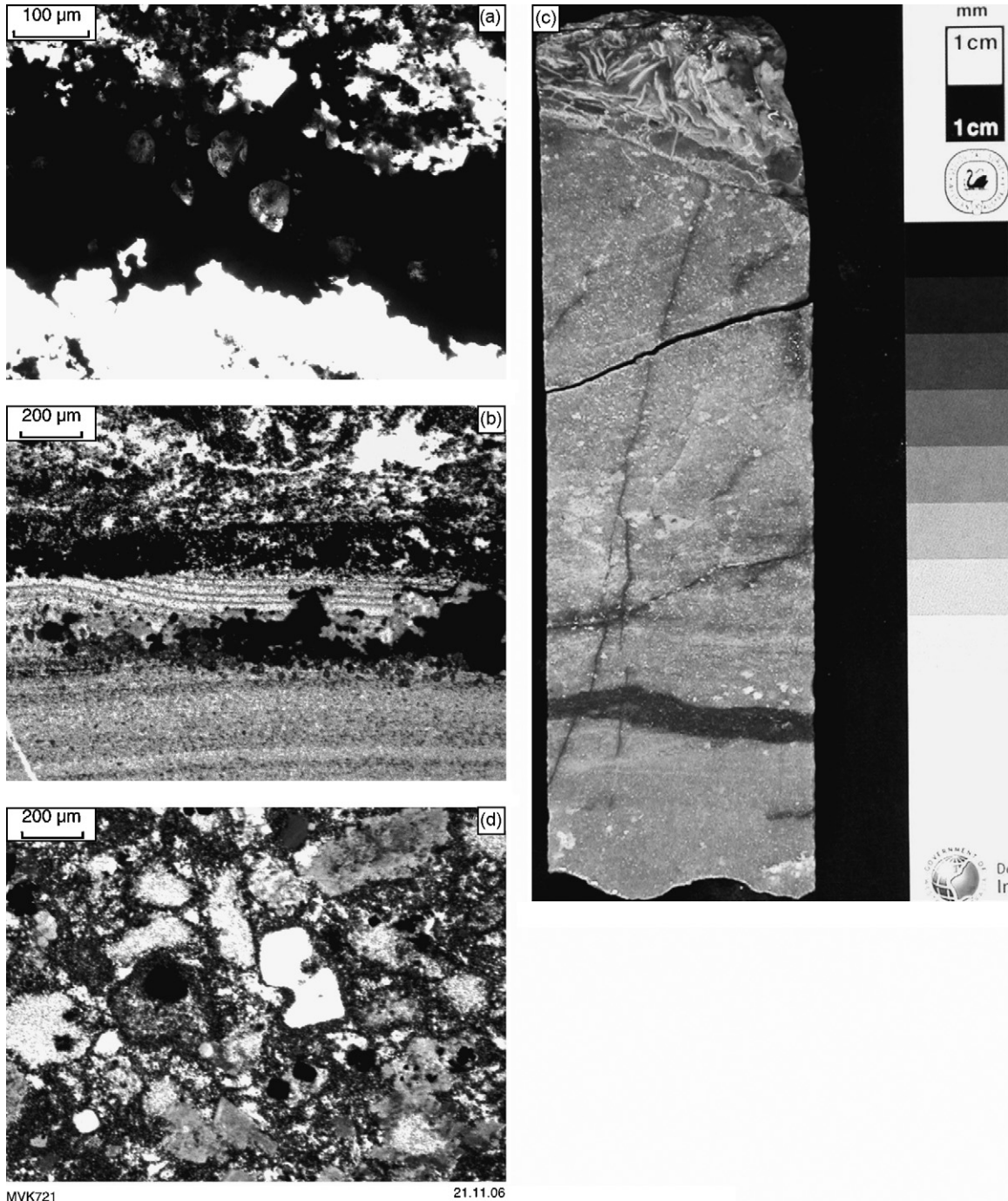
Fig. 13. (a) Plane polarised light thin section view of the unconformity at the base of member 5, showing small euhedral tourmaline crystals encrusted by pyrite (from 94.6 m in PDP2c); (b) plane polarised light thin section view of fine-scale bedding of carbonate rocks of member 6 that are extensively replaced by pyrite (from 94.5 m in PDP2c); (c) drillcore section of the volcanoclastic sandstone sampled for U–Pb zircon geochronology from 94.35 to 94.55 m in PDP2c; (d) cross-polarised thin section view of the silicified volcanoclastic sandstone shown in (c): note the rounded clasts of devitrified felsic volcanic glass (now microquartz and white mica), and the volcanic quartz crystal clast showing resorbed margins.
