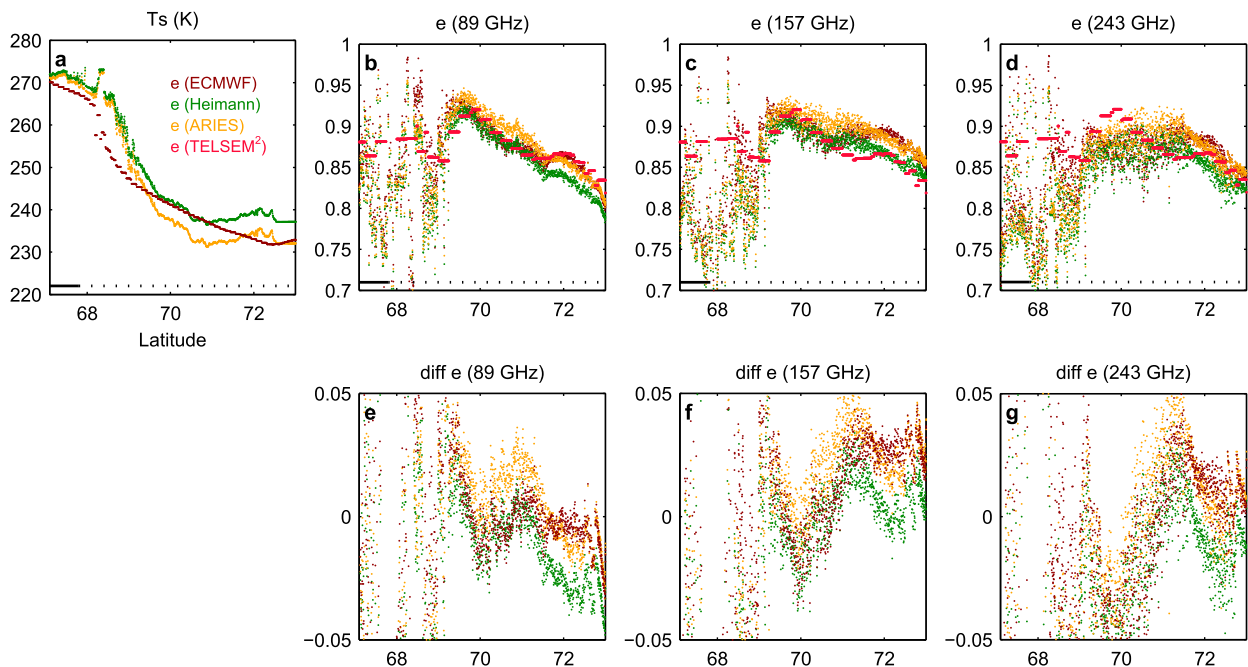
FIG. 14. (a) The surface temperature derived directly from the aircraft observations, along with the ECMWF-Interim database estimates for flight B896 on the way back from Greenland. (b)–(d) The corresponding emissivity at nadir from the aircraft measurements with the different T_s estimates, along with the corresponding TELSEM 2 emissivity. On the x axis, the solid black line indicates the presence of sea ice and the dotted line corresponds to the continent. (e)–(g) The differences between aircraft-retrieved emissivities and the TELSEM 2 emissivity [ e(\text{various airborne}) - e(\text{TELSEM}^2) ]. The brown dots represent e(\text{ECMWF}) - e(\text{TELSEM}^2) , the green dots represent e(\text{Heimann}) - e(\text{TELSEM}^2) , and the orange dots represent e(\text{ARIES}) - e(\text{TELSEM}^2) .
