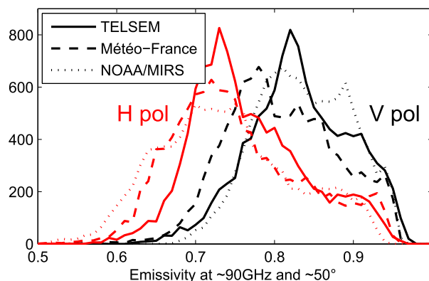
FIG. 3. Histograms of the emissivity around 90 GHz as calculated from the different groups (TELSEM, Météo-France, and NOAA/MIRS) in March over the poles for both polarizations (V in black, H in red). Sea ice surfaces are excluded.
