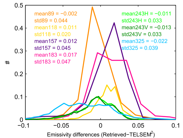
FIG. 16. Histograms of the emissivity differences between the aircraft-derived estimates and TELSEM 2 results, at nadir, over continental ice during flights B896 and B898. Each channel is represented by a different color, and the corresponding statistics (mean and std dev) are provided.
