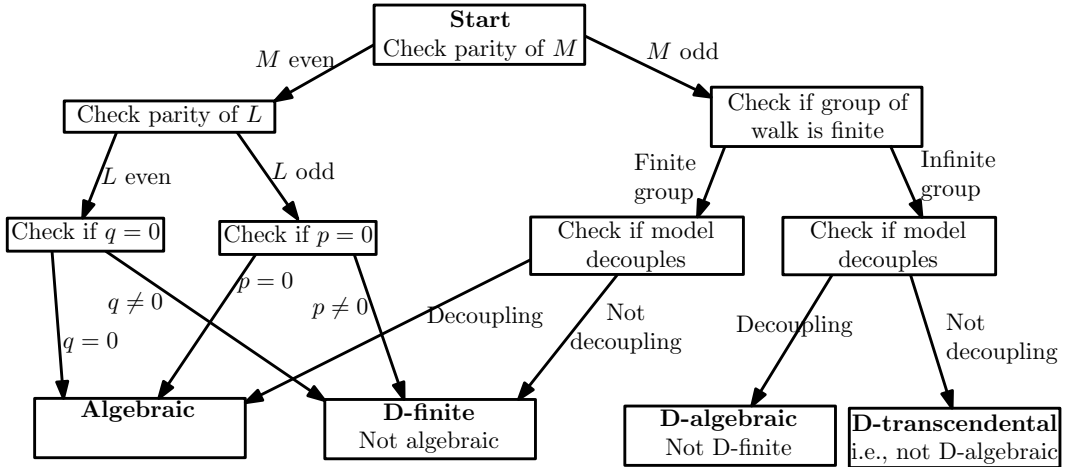
FIGURE 9. A chart showing how to determine the complexity of the series Q_j(x, y; t) counting walks starting at (p, q) confined to an M -quadrant cone as a series in x (or y ) as proven by Theorems 6.2-6.9. Recall that L determines which M quadrants are used to define the M -quadrant cone.
