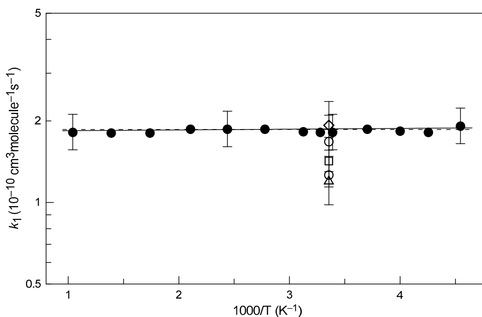
Figure 4. Summary of the measurements of k_1 : diamonds, Williams and Rowland [9]; triangles, Smith et al. [10]; open circles, Schölné et al. [12]; squares, Persky [11]; filled circles, this work. Uncertainties shown for selected present measurements of k_1 correspond to 15%.
