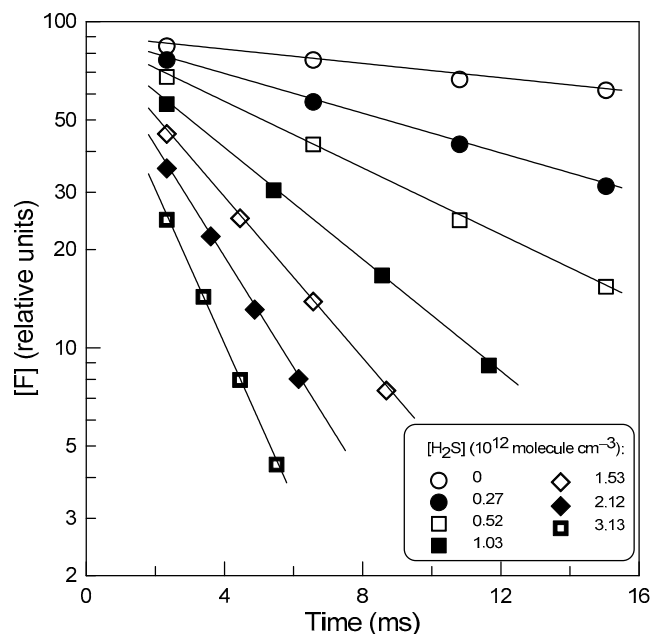
Figure 2. Typical F-atom decay profiles observed in the presence of different concentrations of H_2S at T = 295 K.
