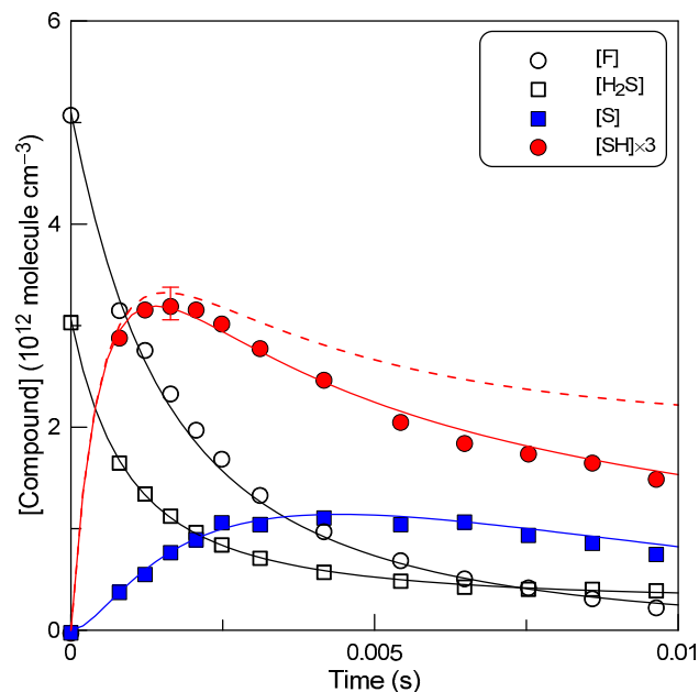
Figure 5. Reaction F + H_2S : measured (points) and simulated (lines) kinetics of the reactants (F and H_2S ) and products (S and SH), T = 295 \text{ K} .
