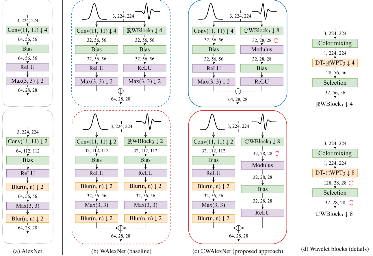
Figure 2. First layers of AlexNet and its variants, corresponding to a convolution layer followed by ReLU and max pooling. The models are framed according to the same colors and line styles as in Figs. 3 and 4. The green modules are the ones containing trainable parameters; the orange and purple modules represent static linear and nonlinear operators, respectively. The bias is represented as a separate module for clarity. The numbers between each module represent the depth (number of channels), height and width of each output. Fig. 2a: freely-trained models. Top: standard AlexNet. Bottom: Zhang’s “blurred” AlexNet. Fig. 2b: \mathbb{R}\text{Max} -based twin models (WAlexNet), reproducing the behavior of standard (top) and blurred (bottom) AlexNet. The 64 output channels are split into two groups. The left side of each diagram corresponds to the 32 freely-trained, presumably low-frequency output channels, whereas the right side (32 remaining channels) represents \mathbb{R}\text{Max}^a (top) or \text{Blur}\mathbb{R}\text{Max}^a (bottom). Both of them contain a wavelet block, whose structure is detailed in Fig. 2d. Fig. 2c: \mathbb{C}\text{Mod} -based twin models (CWAlexNet), where \mathbb{R}\text{Max}^a as well as \text{Blur}\mathbb{R}\text{Max}^a are replaced by standalone \mathbb{C}\text{Mod}^a . Fig. 2d: details of the wavelet block, in its real and complex configurations (respectively, \mathbb{R}\text{WBlock} and \mathbb{C}\text{WBlock} ).
