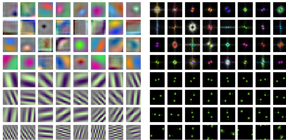
(b) \text{Blur} \circ \text{ReLU} \circ \text{Max}^a (four bottom rows) + Blur
