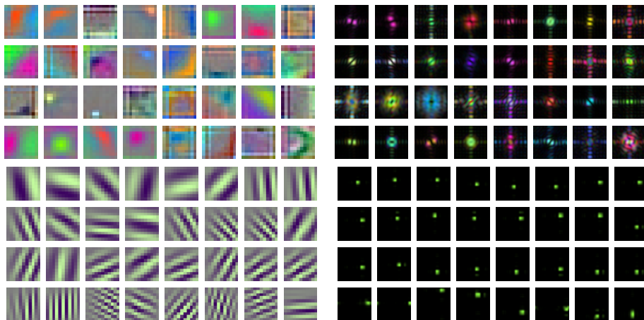
(c) CMod^a (four bottom rows). Spatial domain: real part only
