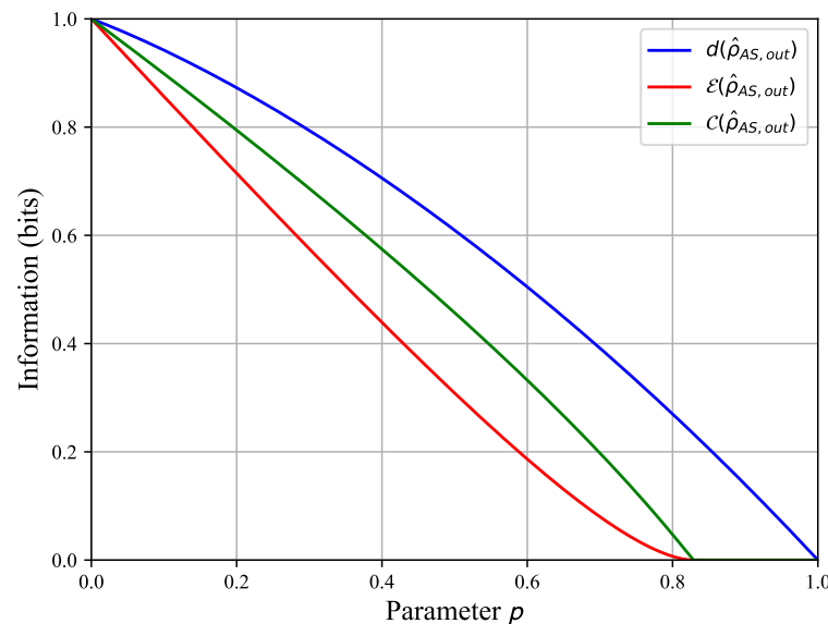
Figure 6. The entanglement rate \mathcal{E}(\hat{\rho}_{AS,out}) (red), the concurrence of Wootters \mathcal{C}(\hat{\rho}_{AS,out}) (green), and the quantum discord d(\hat{\rho}_{AS,out}) (blue) as functions of the parameter p for \xi = 1/2 .
