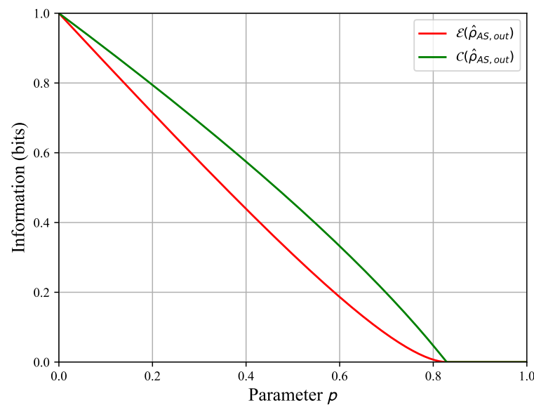
Figure 3. The concurrence of Wootters \mathcal{C}(\hat{\rho}_{AS,out}) in green and the entanglement rate \mathcal{E}(\hat{\rho}_{AS,out}) in red as functions of the parameter p \in [0, 1] for \xi = 1/2 .
