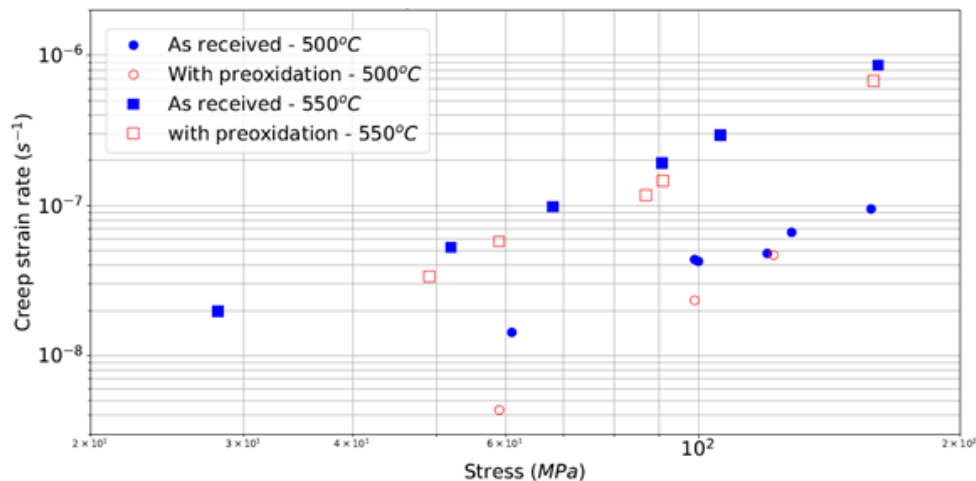
Fig. 7: Norton plot summarizing all the creep tests carried out on as-received and pre-oxidised samples at 500 and 550°C.
