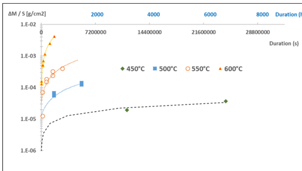
Fig. 2: Oxidation kinetics under laboratory air.
