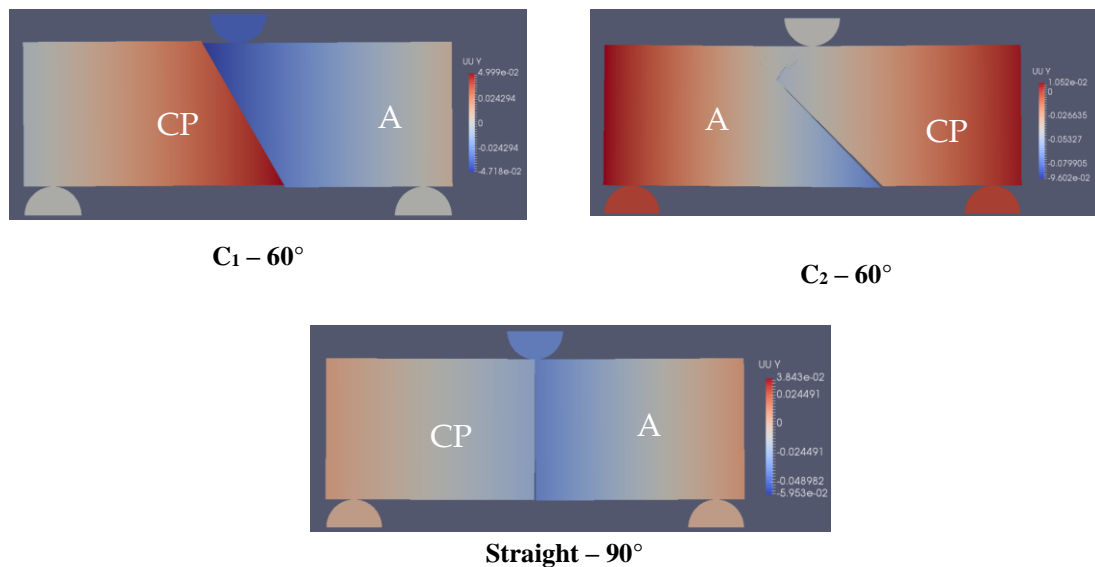
FIGURE 9. Displacement fields of composite specimens subjected to three - point bending with centered load with inclined aggregate ( 30^\circ , 45^\circ , and 60^\circ ) and straight aggregate in two configurations (C1 and C2).
