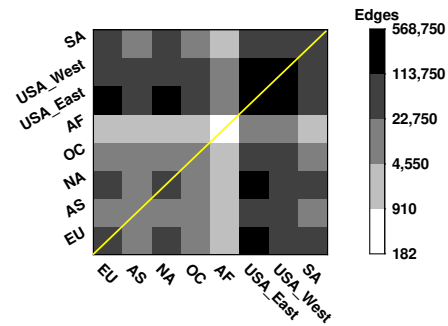
Figure 2 Number of edges between DCs in the Twitter graph, where vertices are located in eight different DCs. SA, AF, OC, NA, AS and EU represent DCs in South America, Africa, Oceania, North America, Asia and Europe, respectively.
