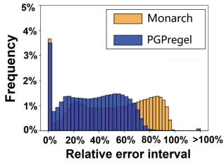
Figure 8 Relative error distribution of a vertex in LiveJournal using PageRank using Monarch and PGPregel.
