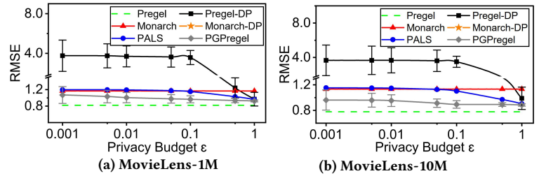
Figure 10 End-to-end accuracy results of compared systems for ALS. Error bars represent standard deviation.
