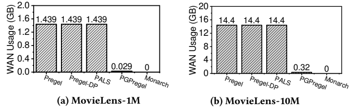
Figure 11 End-to-end WAN usage results of ALS application.
