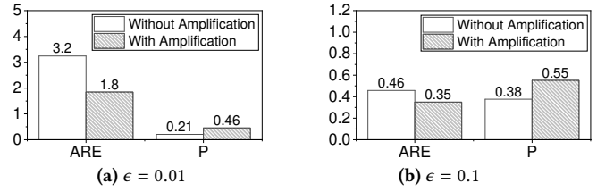
Figure 15 Impact of budget amplification using Livejournal.
