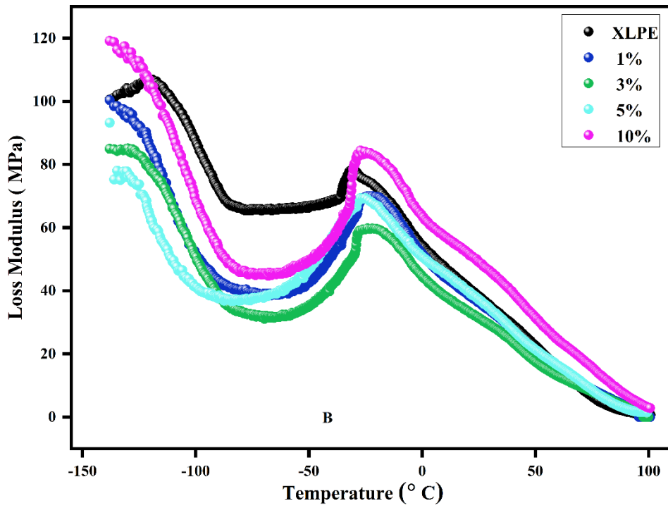
Figure 10 (A) Storage modulus, (B) loss modulus of pure XLPE and its nanocomposites with respect to temperature.
