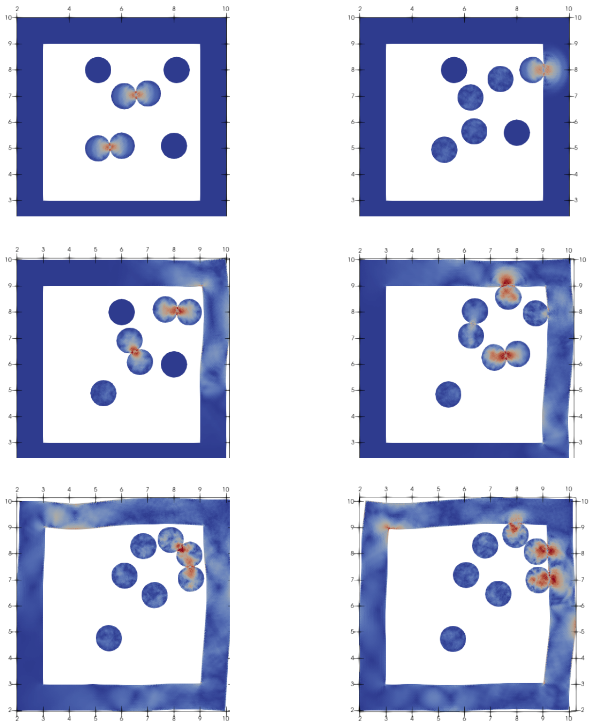
Figure 14: Deformation and multi-contact between solids with color plot of Von Mises stresses at 11 s, 16 s, 20 s, 24 s, 30.5 s and 33 s.
