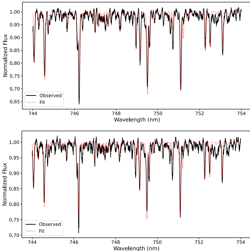
Figure A1. Resulting fit of ZEEMAN synthetic spectra (red) of DQ Tau spectrum (black) over the 744–754 nm range for A ((top) and B (bottom) components.
