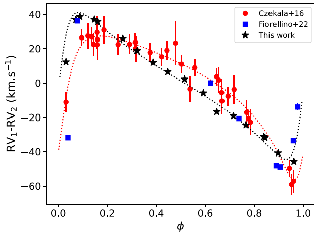
Figure 15. Velocity difference between the primary and the secondary as a function of the orbital phase. The symbols indicate the corresponding publication and the error bars may be smaller than the symbol’s size. The dotted black line is the orbital solution derived in this work. The one in red is the orbital solution found by Czekala et al. 2016.
