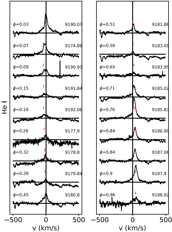
Figure 8. Same as Fig. 4 for He I line at 587.6 nm.
