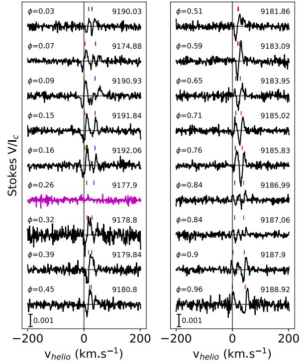
Figure 2. Same as Fig. 1 for LSD Stokes V profiles. As the observation at \phi = 0.26 (magenta) exhibits a poorer S/N, we divided this profile (only) by 10 for more visibility.
