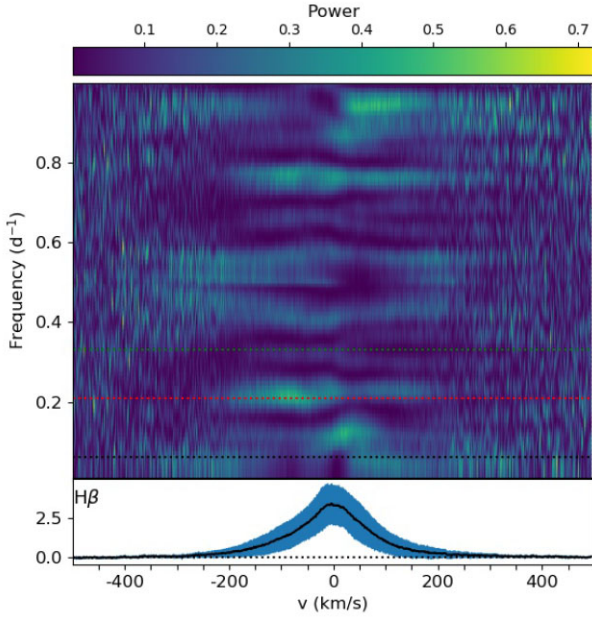
Figure 7. Same as Fig. 6 for the residual H \beta line.
