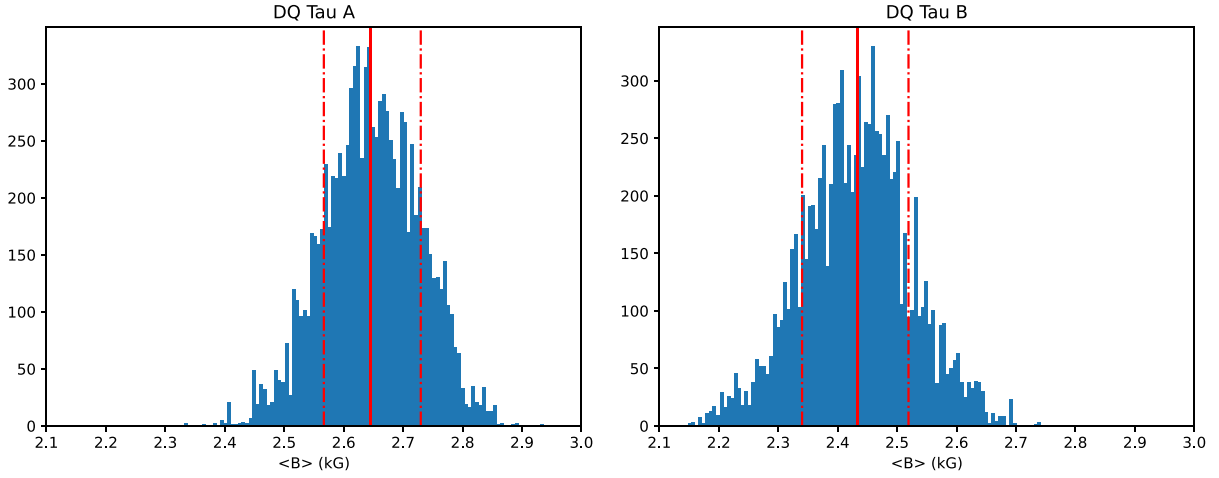
Figure 13. Posterior distribution of the surface-averaged magnetic field strength from the Zeeman intensification analysis for A (left) and B (right) components of DQ Tau. The solid vertical line represents the median value and the dash dotted ones represent the 68 per cent confidence intervals.
