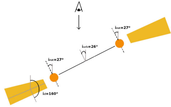
Figure 16. Sketch representing the inclination angles of the components’ rotation axis, the orbit rotational axis, and the disc’s plane as used in this work. The eye with the arrow indicate the line of sight, the orange circles represent the two components and the dashed lines their rotation axis. The black line between them is the orbital plan and the disc is represented by the yellow part on each side. The grey lines are guiding the angle visualization.
