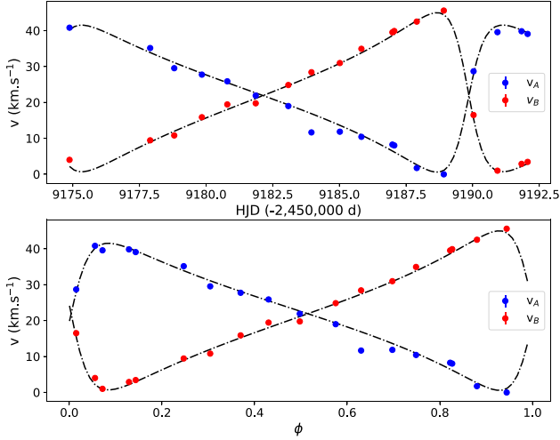
Figure 3. Radial velocities of the primary (A, in blue) and secondary (B, in red) component of the DQ Tau system, determined from the LSD Stokes I profiles, as a function of HJD ( top ), and the orbital phase ( bottom ). The error bars are provided but smaller than the symbol size. The black dash-dotted curve is the orbital solution derived in this work, with the parameters provided in Table 3.
