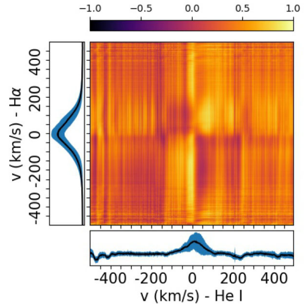
Figure 10. Correlation matrix of H \alpha vs. He I lines. The colourmap illustrates the correlation coefficient: Light yellow for a strong correlation (i.e. close to 1) and dark purple for a strong anticorrelation (i.e. close to -1 ). The panels along the x - and y -axis display the mean He I and H \alpha profiles, respectively, in black, with their variance in blue.
