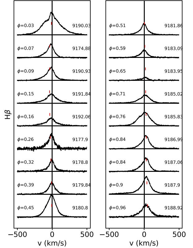
Figure 5. Same as Fig. 4 for the residual H\beta profiles.
