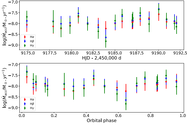
Figure 11. Mass accretion rate computed from H \alpha (red), H \beta (blue), and H \gamma (green) residual profiles as a function of HJD (top) and the orbital phase (bottom).
