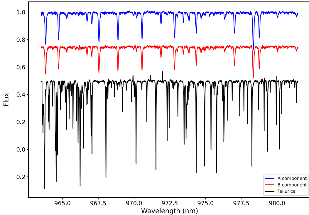
Figure C1. Disentangled spectra of the 963.5–981.5 nm region. The spectra of the A (blue), B (red), and tellurics (black) components have been shifted vertically for more visibility.
