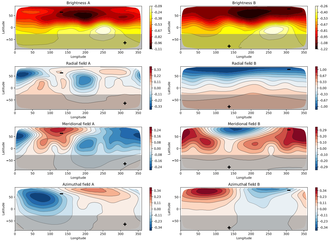
Figure 12. ZDI magnetic field maps of the A component (left), and B component (right). The 0-latitude represents the stellar equator, 90^\circ and -90^\circ the North and South rotational poles, respectively. The 0– 360^\circ longitudes scale the phases 0 to 1 of the stellar rotation cycle. The grey-shaded areas represent the unseen region of the stellar surface due to the stellar inclination given in Table 4. The ‘+’ and ‘-’ signs are locating the dipolar positive and negative pole, respectively. Top panels: Brightness maps, the colour bar indicates the logarithm of the normalized brightness. Three bottom panels: Radial, meridional, and azimuthal fields. The colour bar is in units of \log(kG) .
