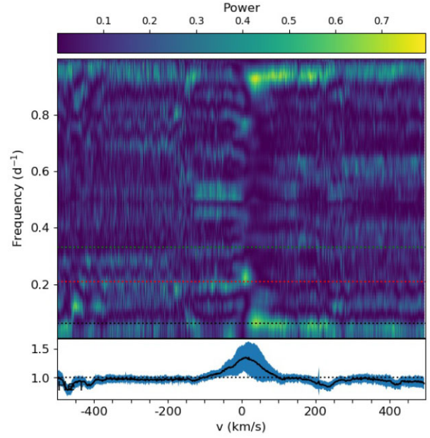
Figure 9. Same as Fig. 6 for He I line at 587.6 nm.
