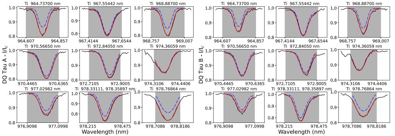
Figure 14. Observed Ti I lines used for the Zeeman intensification analysis (black) and the spectrum synthesis fits corresponding to the optimal parameters (red) for A (left) and B (right) components. The dashed blue lines correspond to the spectra without magnetic field. The grey area represents the region where the fit is performed and the central wavelength of each line is given at the top of each panel.
