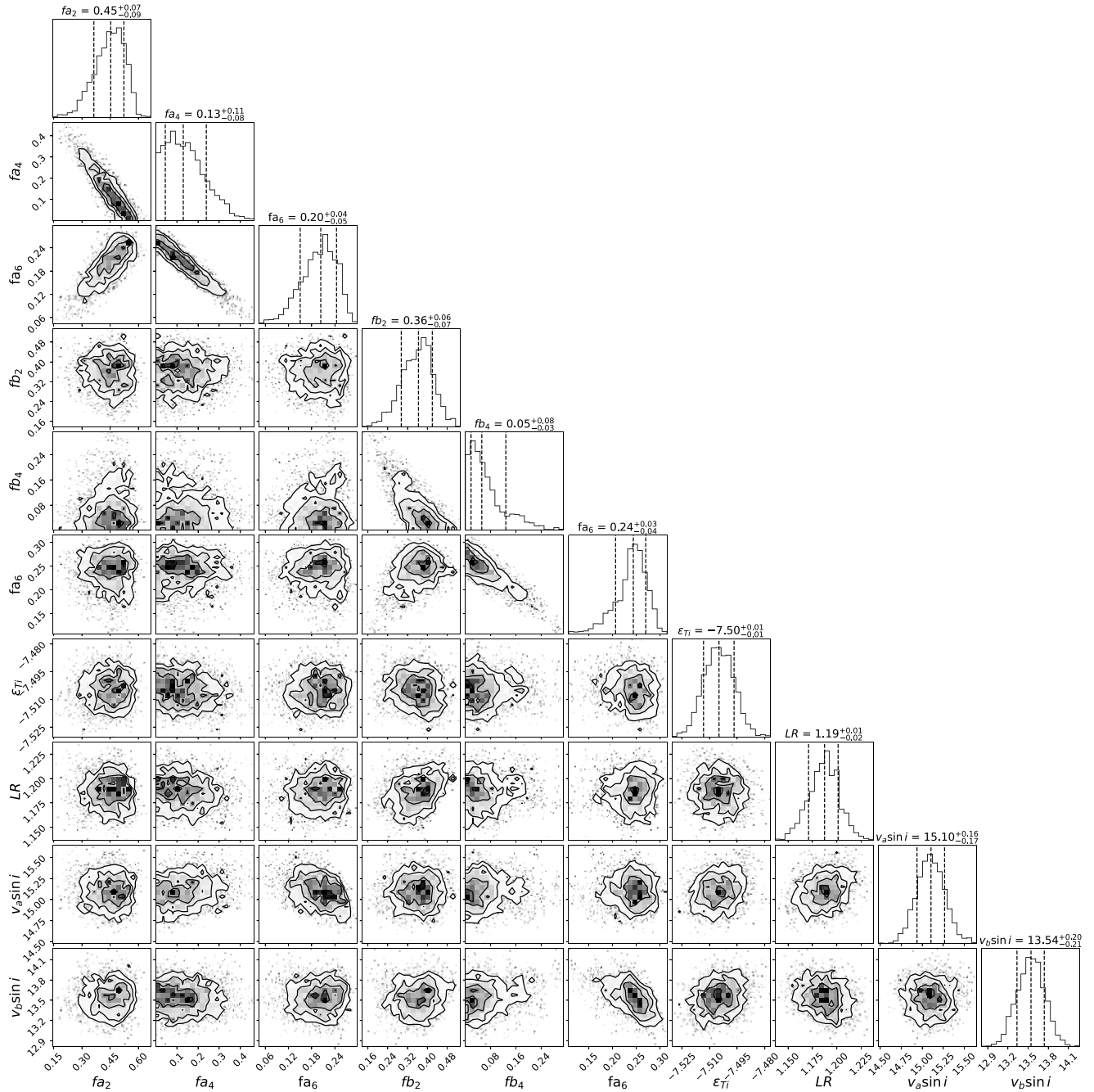
Figure D1. Corner plot showing the posterior distribution of the parameters derived by the Zeeman intensification analysis. From left to right: Filling factors of the 2, 4, and 6 kG magnetic field strengths for A and B components, Ti abundances, luminosity ratio, and v \sin i values for the A and B components.
