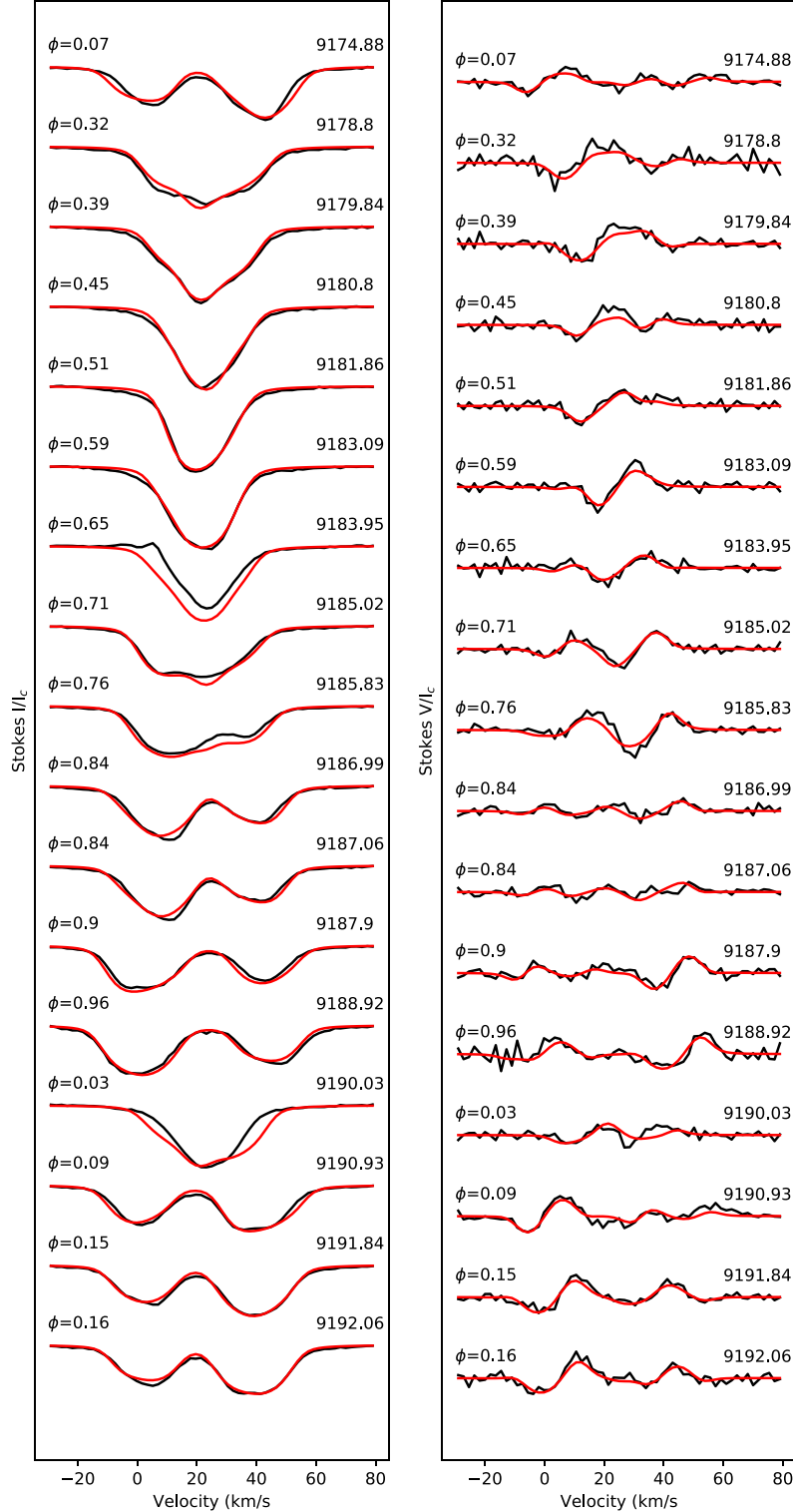
Figure B1. LSD Stokes I (left) and V (right) profiles analysed with ZDI analysis (black) and the resulting model fit (red).
