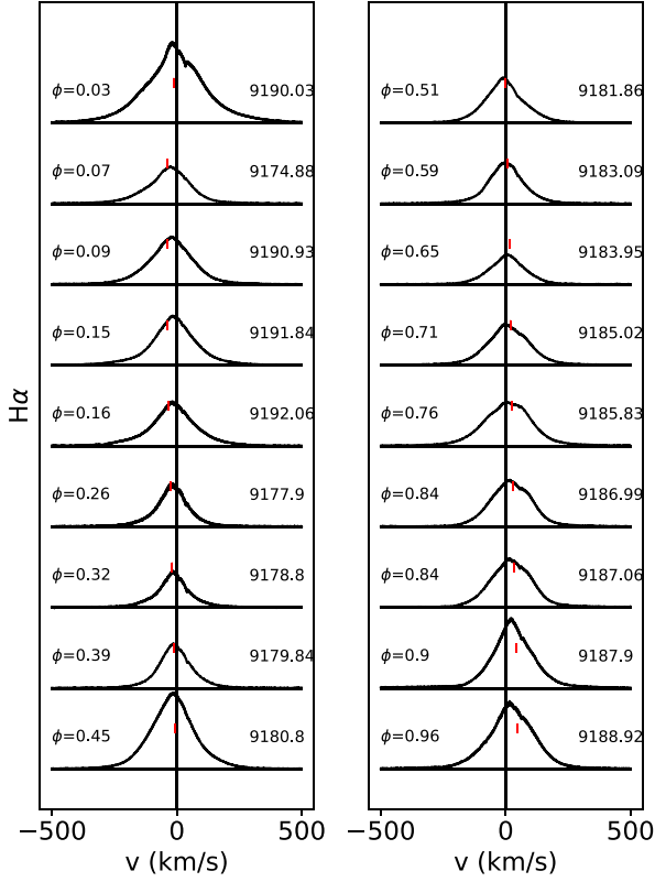
Figure 4. Residual H\alpha profiles centred on the primary’s radial velocity. The vertical line illustrates the 0 velocity and the red ticks indicate the radial velocity of the secondary. The orbital phase is indicated at the left of each profile and the HJD of observation is indicated on the right.
