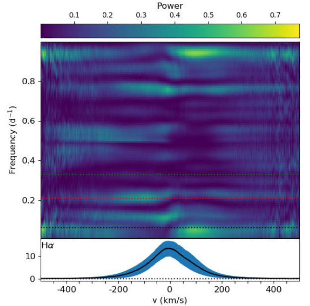
Figure 6. Top: 2D periodogram of the residual H\alpha line. The colour bar goes from dark blue, for the lowest periodogram’s power, to light yellow for the highest. The three horizontal dotted lines indicate the rotation period of the primary at 3.03 d (green), the orbital period at 15.8 d (black) and an unexpected signal at f \sim 0.21 \text{ d}^{-1} or 4.8 d (red). Bottom: Mean profile (black) and its variance (blue).
