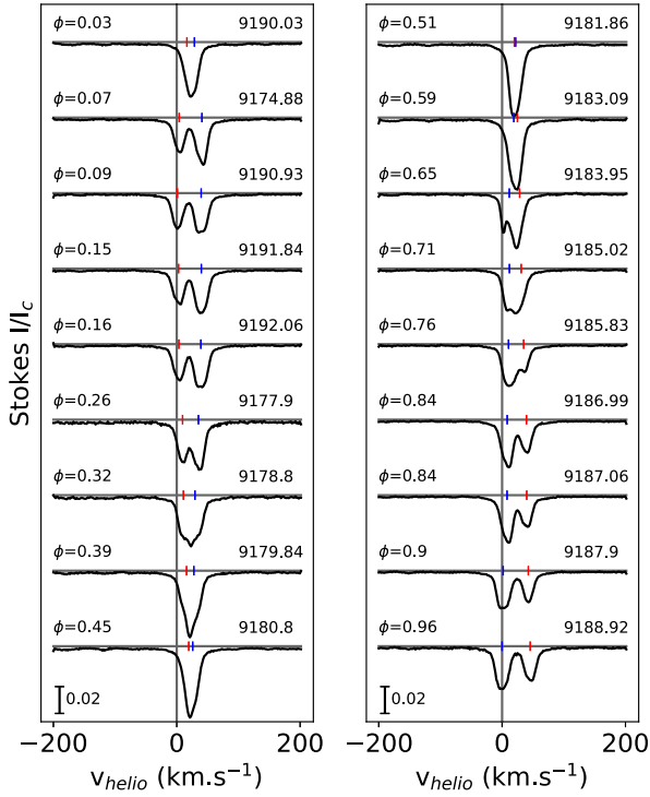
Figure 1. LSD Stokes I profiles of DQ Tau system. The orbital phase of each observation is indicated at the top left of each profile, and the HJD ( -2\,450\,000 d) at the top right. The vertical line indicates the 0 velocity. The blue and red ticks indicate the radial velocity of the A and B component, respectively.
